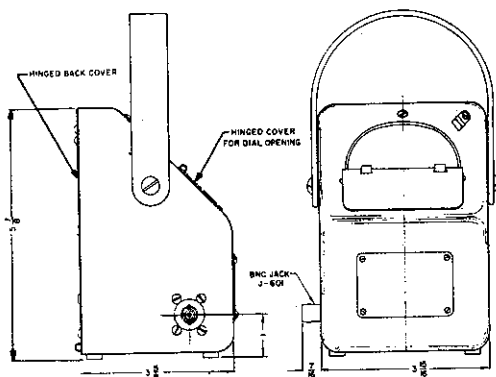
Fig. 3-1 Outline Drawing, Model 6254 Wattmeter
