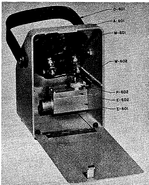
Fig. 4-1 Parts Identification Photograph
