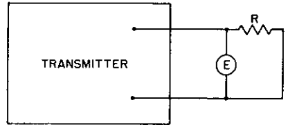
Fig. 2-1 Circuit Diagram E^2/R Method of Power Measurements
