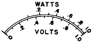
Fig. 2-2 Square Law Scale, Watts vs. Volts
