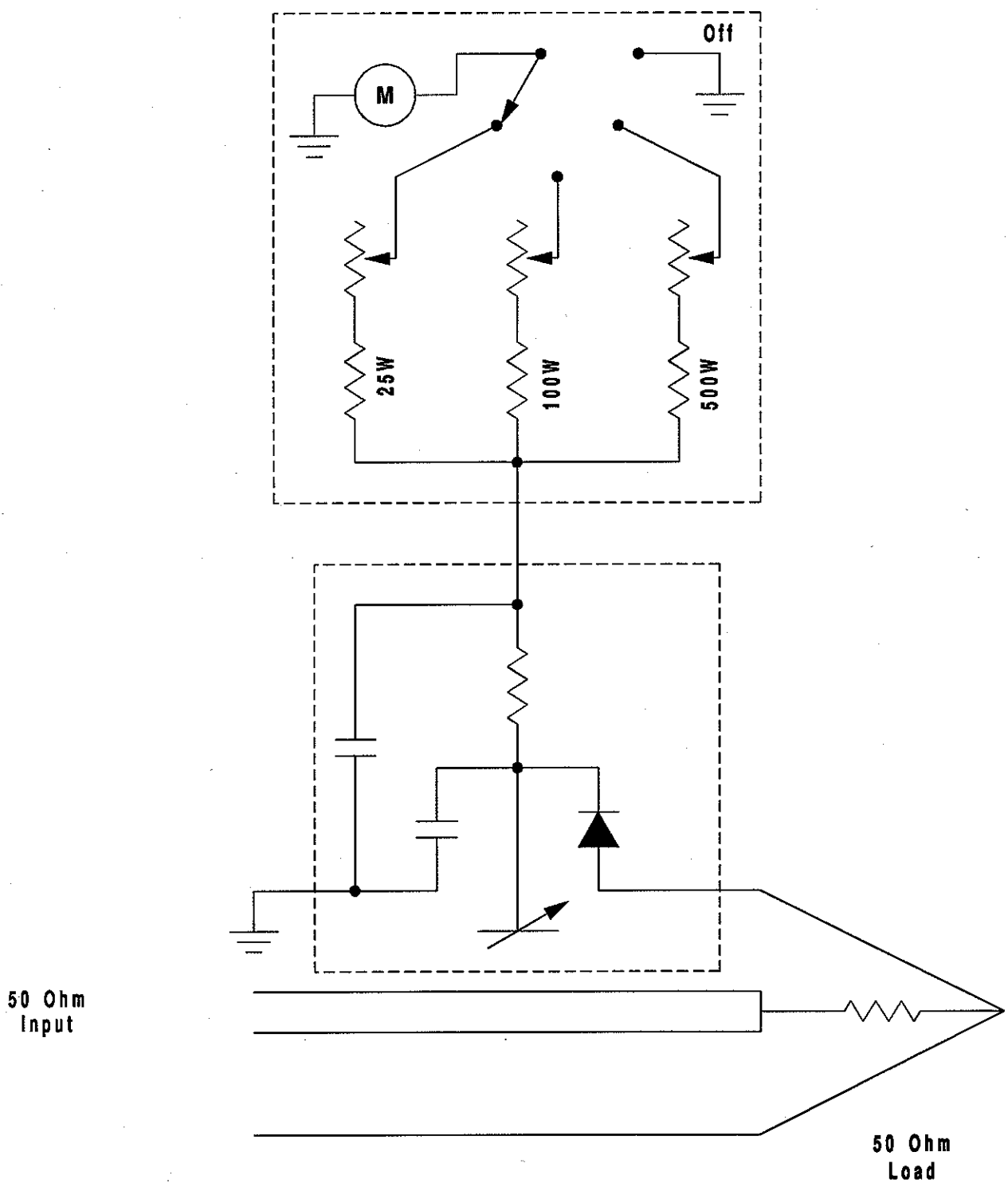
Figure 2-1. Schematic Diagram for Models 6734A-030, 6736-030A, 6737-030A.
