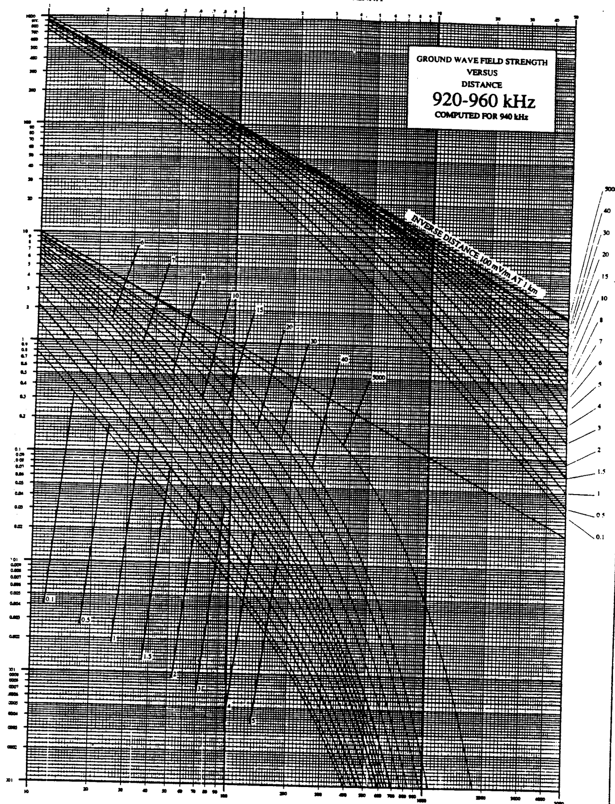
KILOMETERS FROM ANTENNA GRAPH 11
