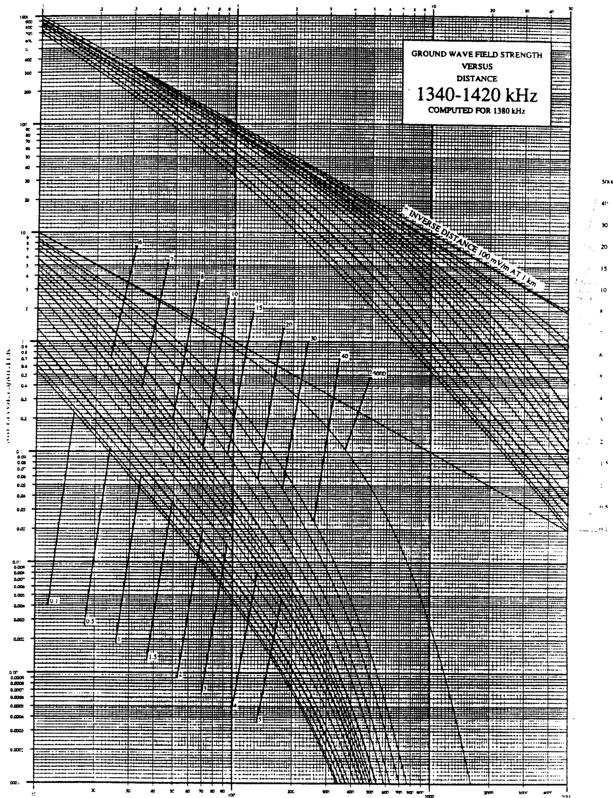
KILOMETERS FROM ANTENNA GRAPH 17
