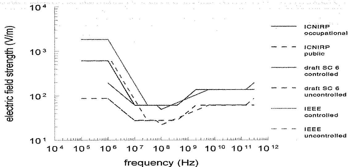
Figure 4.2-3: Comparison of power density reference levels in SC6 (2013) with international standards
