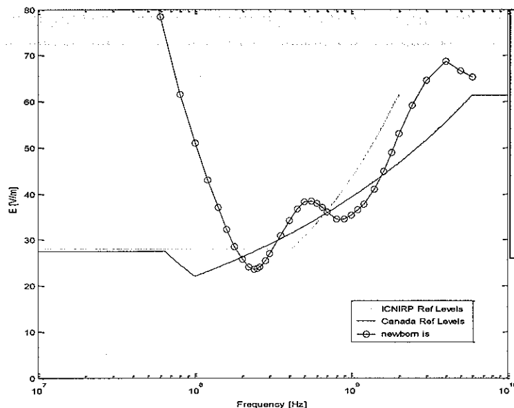
Figure 6.4-10: Electric field strength values required to produce Health Canada SC6 (2013) basic restrictions on WBSAR for a newborn model under isolated conditions for uncontrolled environments between 10 MHz and 10 GHz (Dimbylow, 2010).
