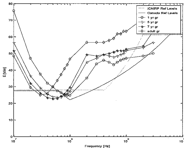
Figure 6.4-7: Electric field strength values required to produce Health Canada SC6 (2013) basic restrictions on WBSAR for male adult and child models in the standing (arms up) postures under grounded conditions for uncontrolled environments between 10 MHz and 10 GHz (A-K Lee et al., 2012).
