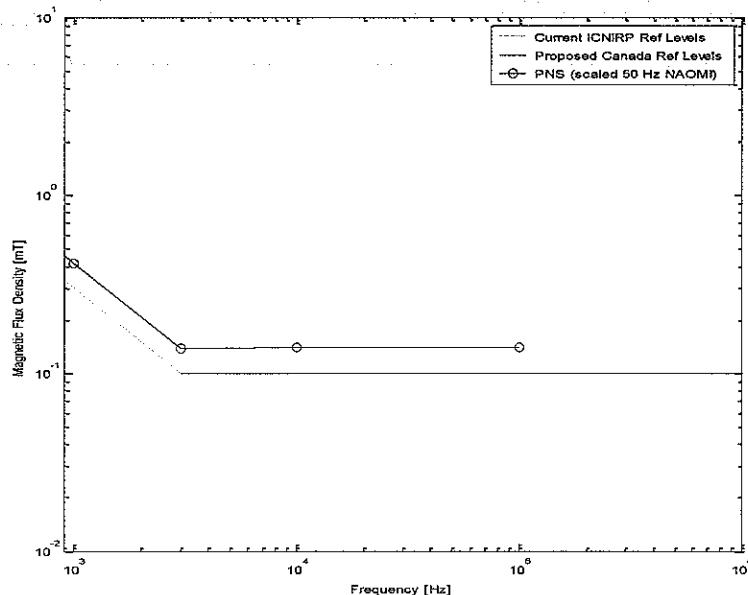
Figure 6.4-3: External magnetic flux density values required to produce the proposed controlled environment basic restriction for PNS as a function of frequency for the female adult NAOMI phantom (Dimbylow 2005) and a standard skin conductivity of 0.1 \text{ S m}^{-1} .
