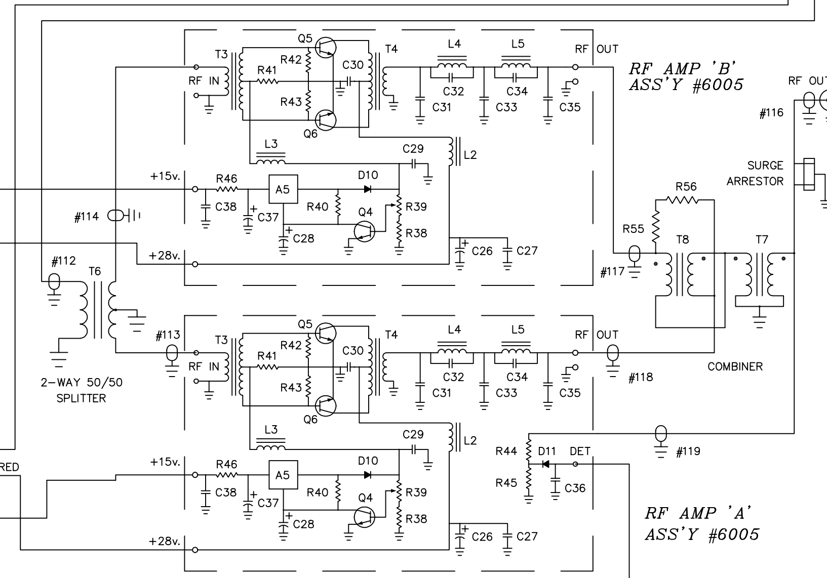
AM-60TIS MAIN FRAME SCHEMATIC #6127 REV.A
