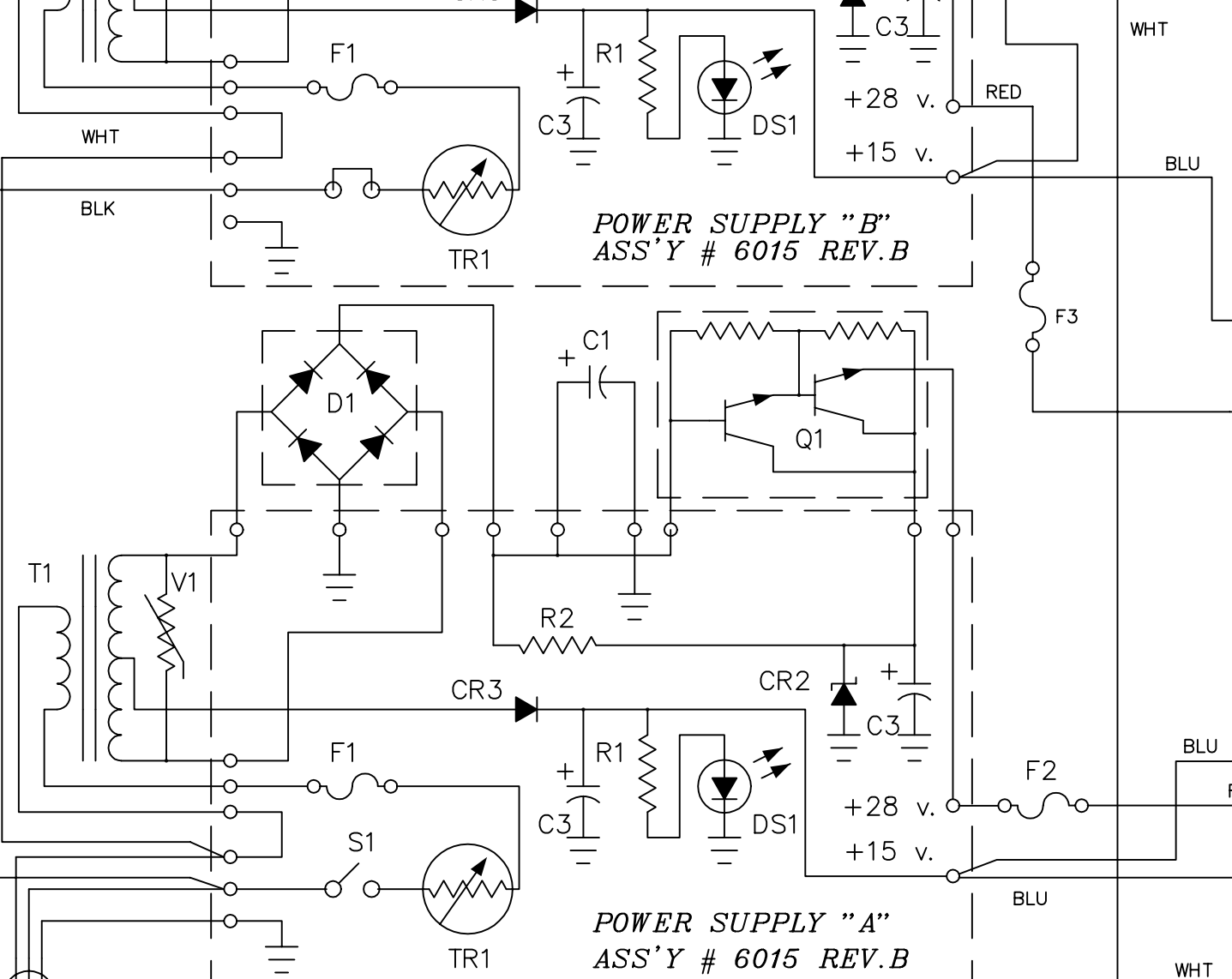
AM-60TIS MAIN FRAME SCHEMATIC #6127 REV.A
