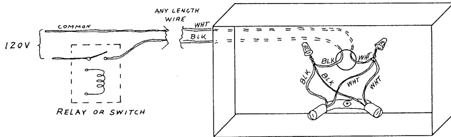
PARALLEL CONNECTION FOR 120 VOLTS
