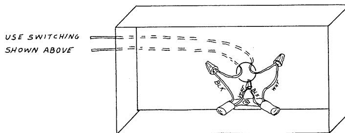
SERIES CONNECTION FOR 240 VOLTS
