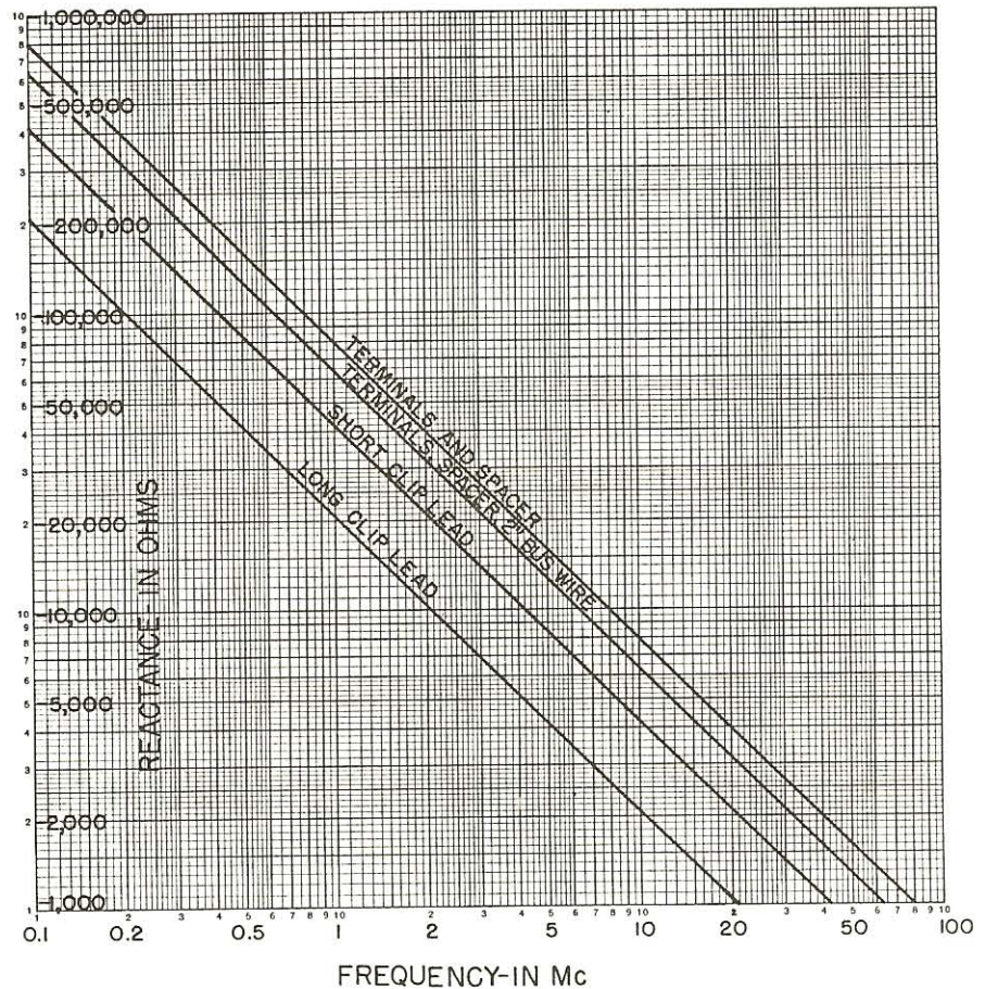
Figure 6. Capacitive Reactance to Ground of Connecting Leads as a Function of Frequency.
