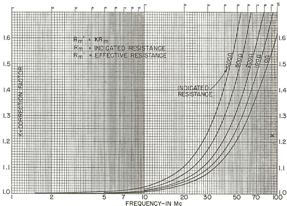
Figure 7. Multiplying Factor for RESISTANCE Dial as a Function of Frequency and Dial Setting (for use with 7-in. connecting lead).
