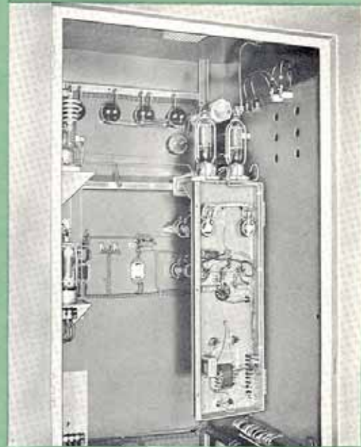
ABOVE—Audio portion of transmitter is on hinged chassis allowing instant servicing of under chassis components not usually readily accessible in other transmitters.
