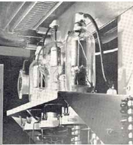
The final amplifier and modulators are in the illustration above. A single type 450TH or 250TH may be used for the final amplifier without making any mechanical or electrical changes. The modulators are 810 tubes.
