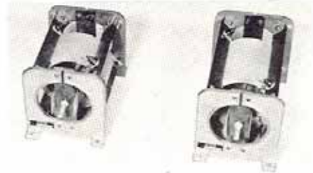
Gatesway variable edgewise coils
