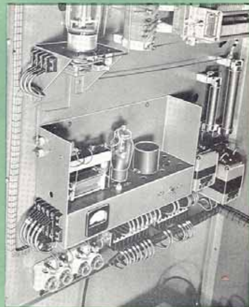
BELOW—Oscillator chassis, completely plug-in and quickly removable in case of urgent servicing. Only one oven shown, but two supplied. Crystal change-over switch is on this chassis also. Dust cover has been removed for this illustration.
