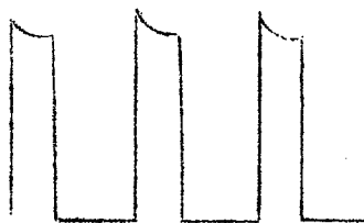
Fig. 6, Typical Waveform, Output V102
