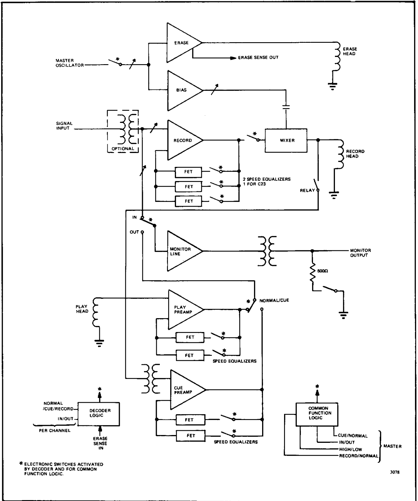
Figure 5-4. Signal Electronics
