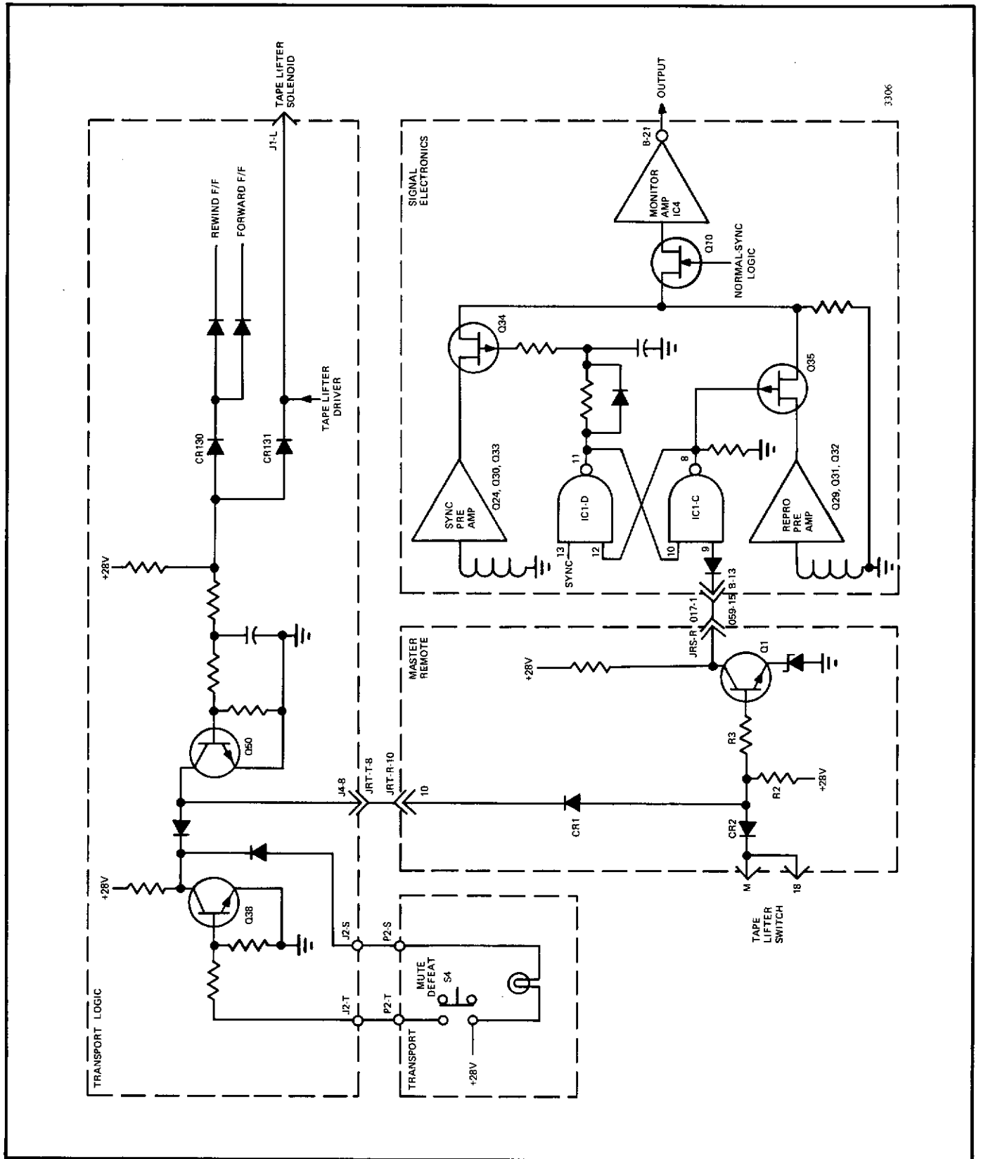
Figure 5-2. Mute Defeat Circuit
