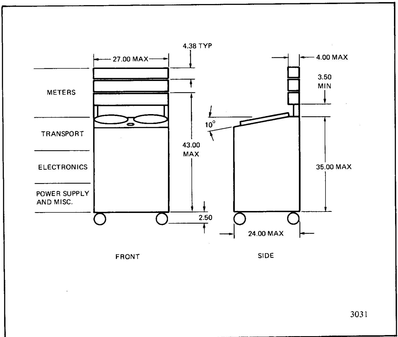
Figure 2-1. Outline Dimensions
