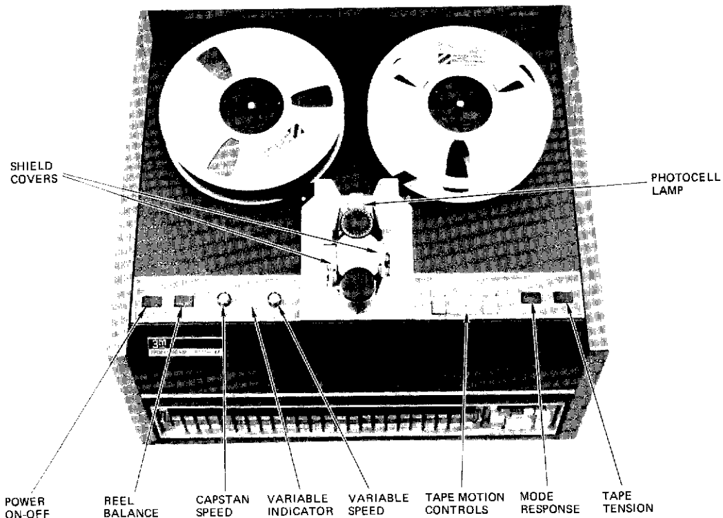
Figure 3-1. Operating Controls
