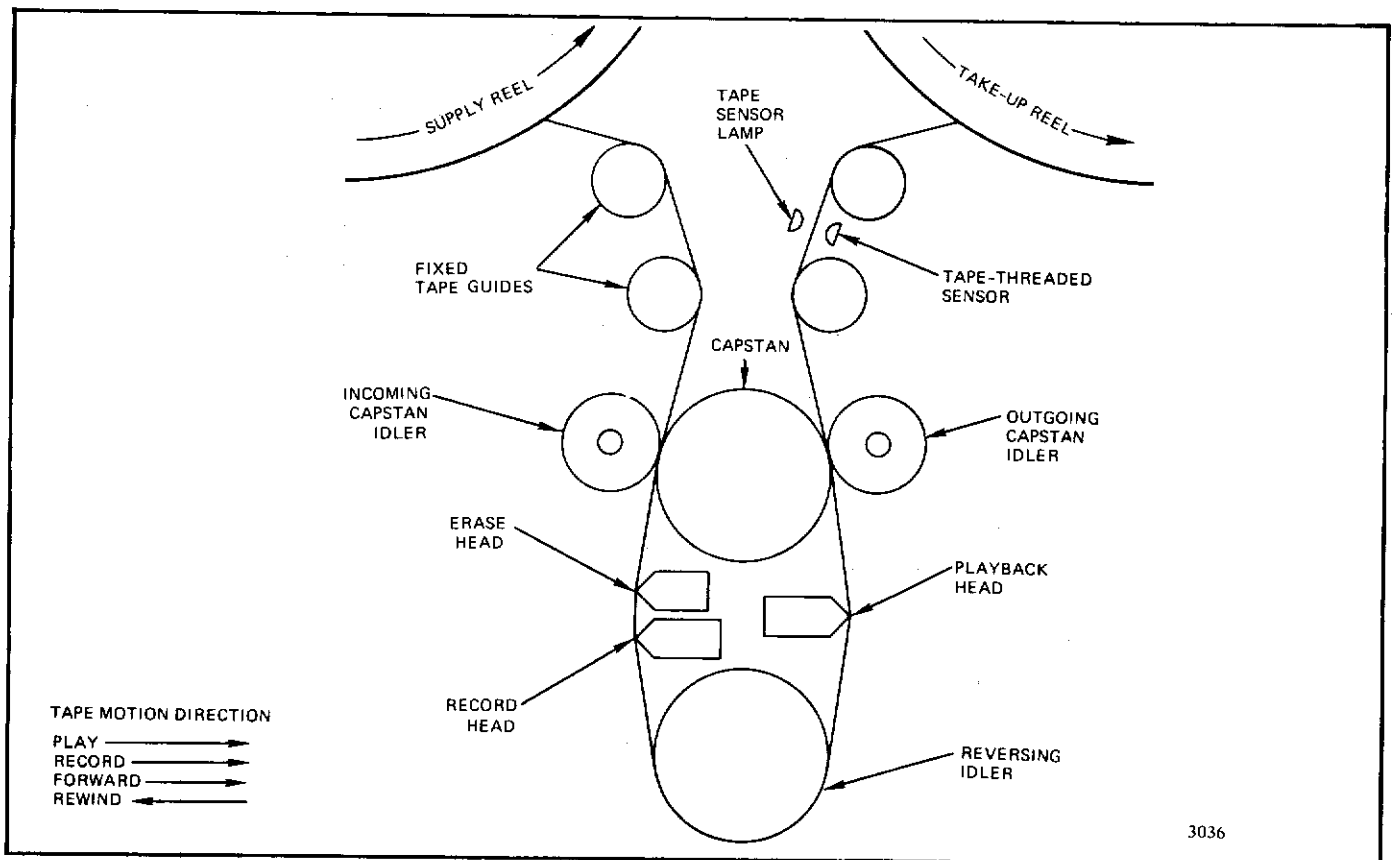
Figure 3-3. Tape Threading
