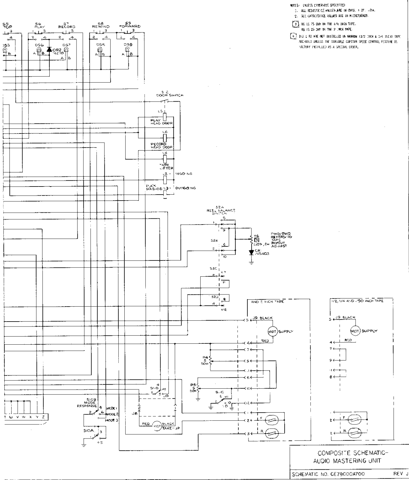
Figure 6-1. Composite Schematic
