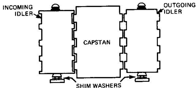
Figure 4-3. Capstan Idler Alignment
