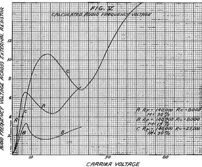
Fig. 5. Audio-frequency voltage.
