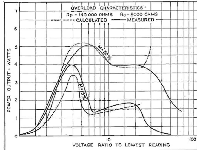
Fig. 6. Overload characteristic.
