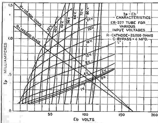
Fig. 7. Ip-Eb characteristics when 25,000-ohm cathode resistor used.
