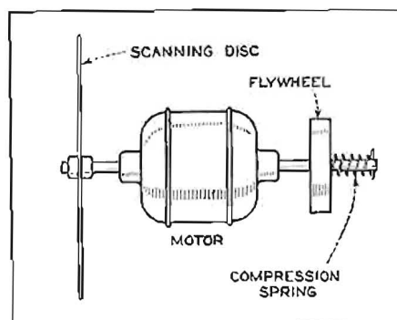
Fig. 1. Disc drive.
