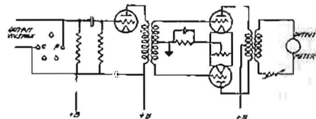
Fig. 1. Circuit for test.
