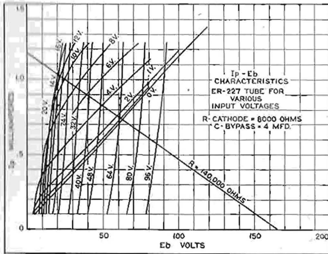
Fig. 3. Characteristics of 227 tube.
