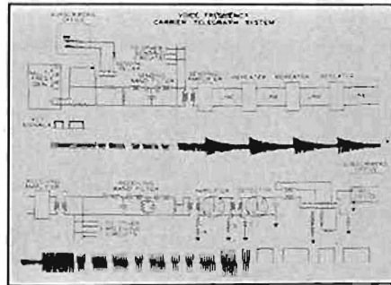
Fig. 7. Voice frequency telegraph system.
