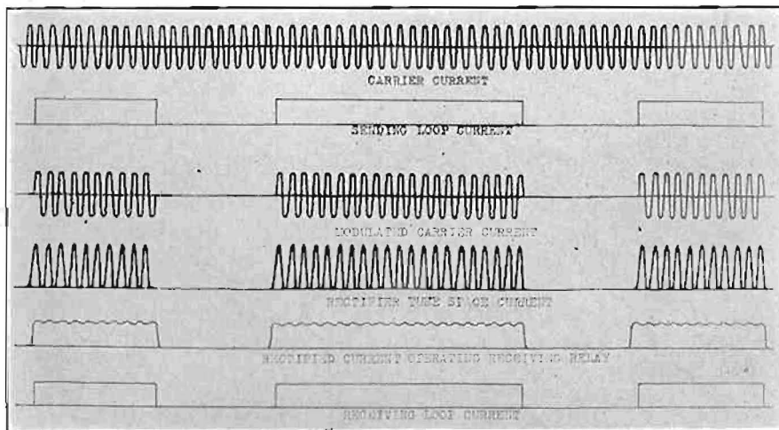
Fig. 2. Type B carrier telegraph. Modulation and demodulation.
