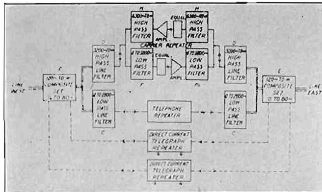
Fig. 6. Type B carrier telegraph. Repeater connections.
