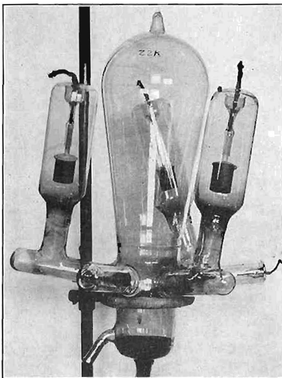
Fig. 1. High voltage mercury cathode tube.
