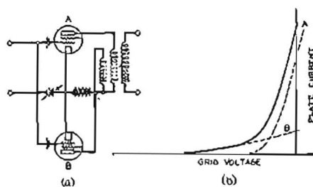
Fig. 2. Method of decreasing distortion and cross-talk.
