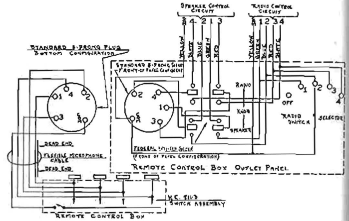
Fig. 4. Remote control box and outlet panel.
