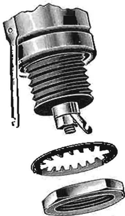
Grounded Can Mounting
