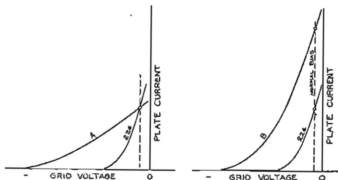
Fig. 1. Showing (a) decreasing transconductance and (b) increasing plate current accompanying attempts to decrease distortion by decreasing the mu-factor.
