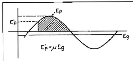
Fig. 3. Only the hatched portion of cycles is passed when E_g is applied. The amount of energy passed by the tube can thereby be controlled.
