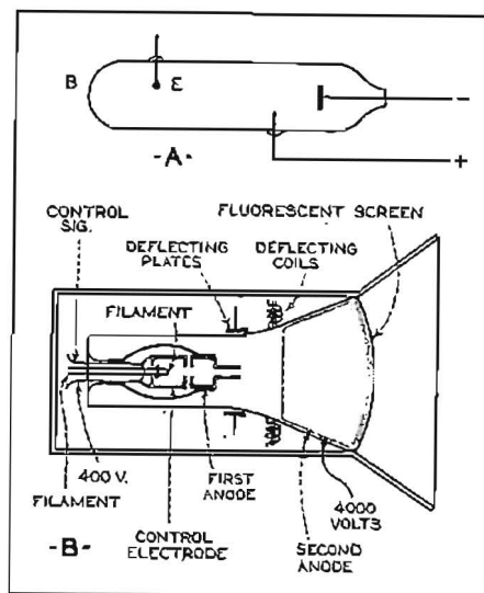
Fig. 1. Cathode ray tube, theory and construction.
