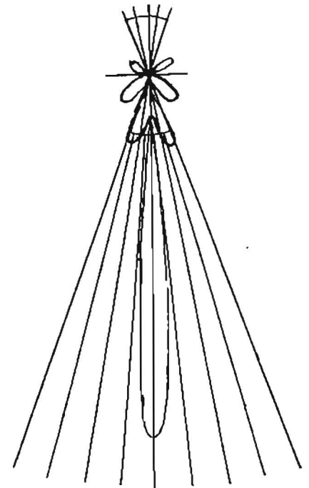
Fig. 11B. Polar diagram for Grecian curtain antenna system.
