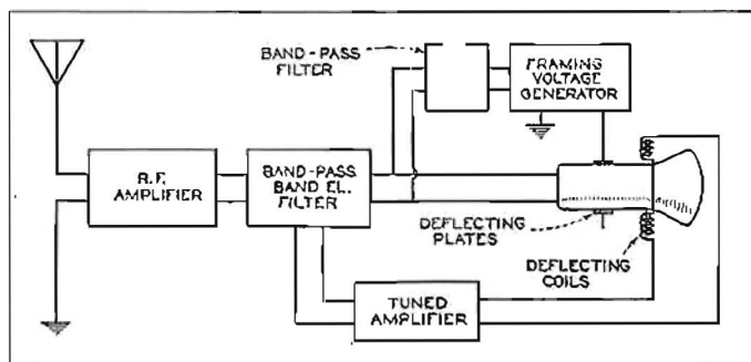
Fig. 2. Unit layout of television receiver.
