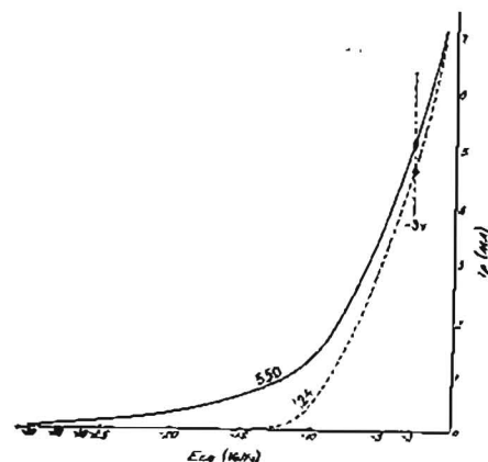
Fig. 6. Plate current-grid voltage characteristic of variable-mu tube showing reshaped characteristic for reduction of distortion and cross-talk.
