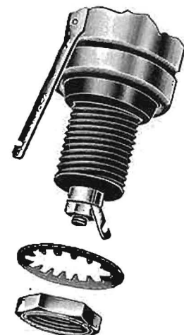
Insulated Can Mounting
