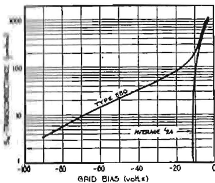
Fig. 7. Transconductance-grid voltage characteristic of Types 550 and -24 tubes.
