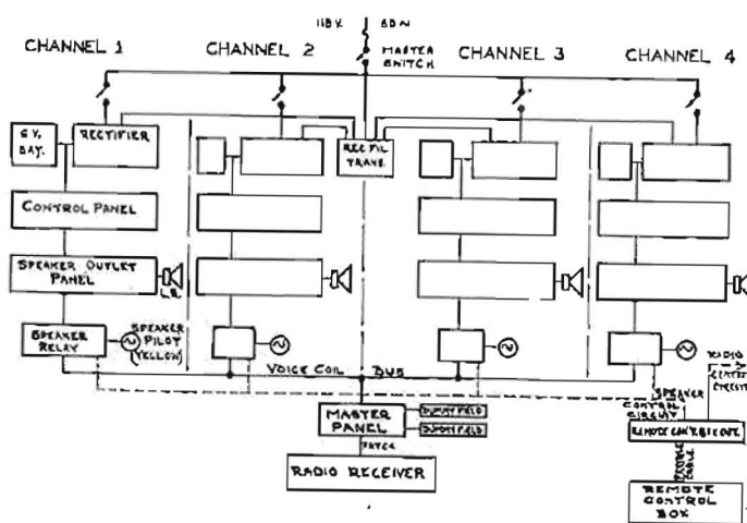
Fig. 5. Schematic diagram loud-speaker comparison circuit.
