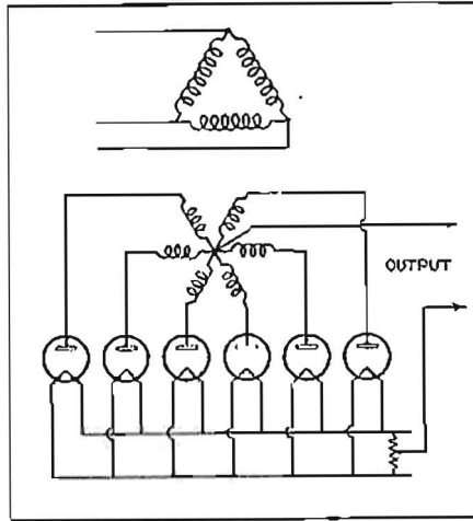
Fig. 2. Six-phase rectifier, employing six tubes.
