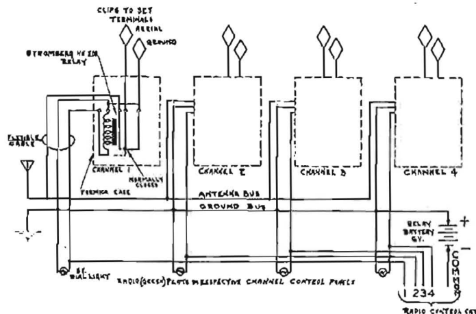
Fig. 2. Wiring diagram antenna relay switching system.
