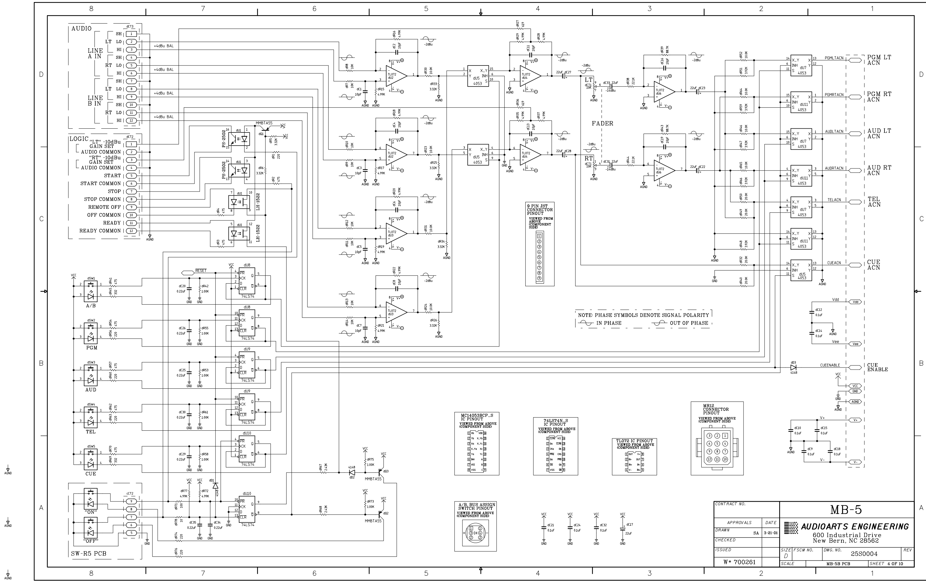
MB-5 Mother Board (Line Input Section "d") Schematic - Sheet 4 of 10
