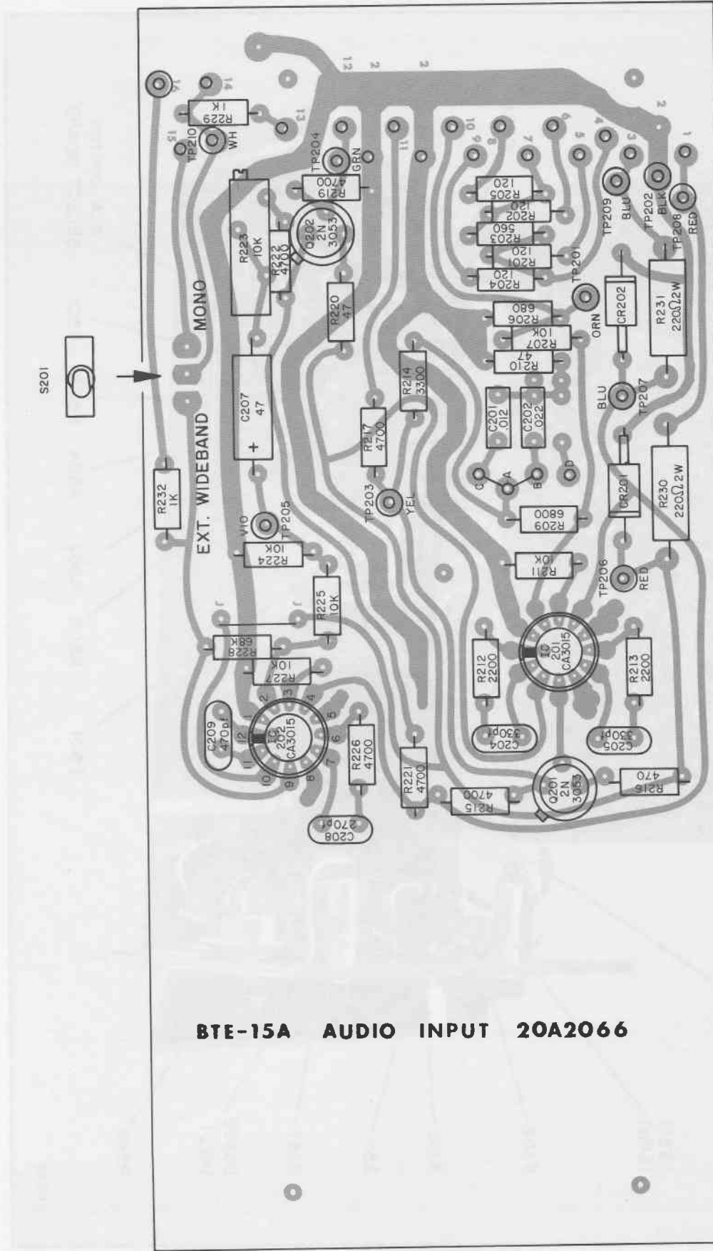
Figure 39. Monaural Audio Board, Parts Overlay, Bottom
