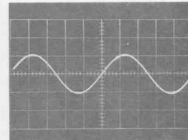
Junction of L301 and R325; Pilot Signal 1 V/cm, 10 \mu\text{sec}/\text{cm} Sync: Ext. from TP304
