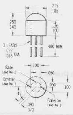
2N3640
