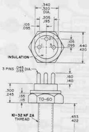
2N4440 2N5102
