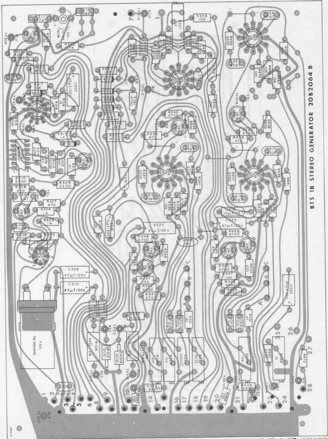
Figure 35. Stereo Generator Board, Parts Overlay, Bottom
