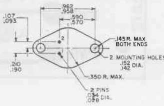
2N3054 2N3740
