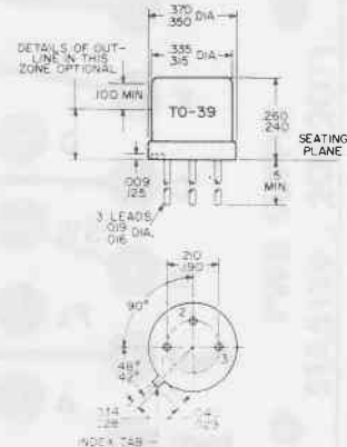
2N4427 2N3866
