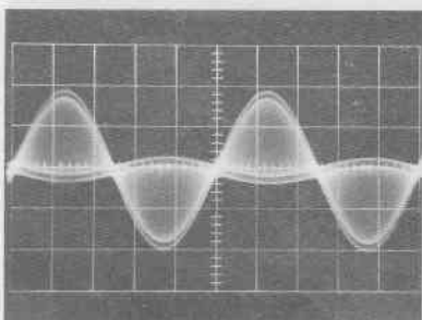
TP411 (white); Composite Output 1 V/cm, .5 ms/cm Sync: Ext. audio generator Waveform showing excessive amplitude of L-R signal.
