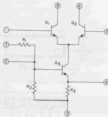
CA3028A
