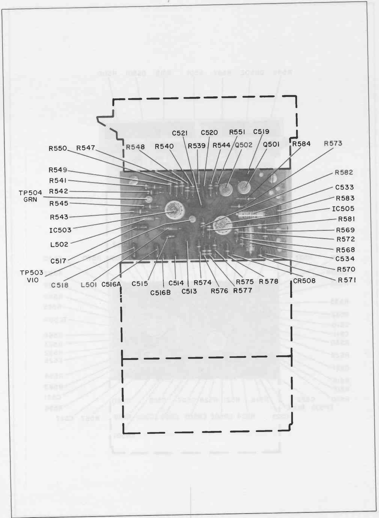
Figure 41. SCA Generator Board, Parts Location, Ser. No. 1 through 999
