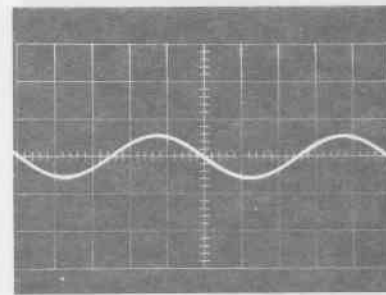
*TP410 (yellow); 17 kHz Filter Output 1 V/cm, .5 ms/cm Sync: Ext. audio generator
