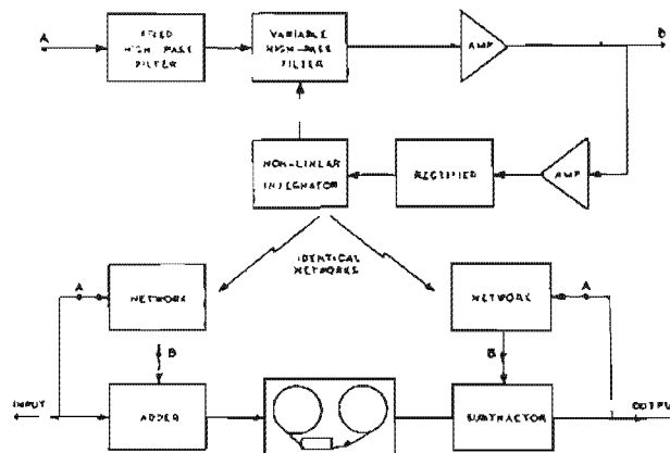
Block diagram of B-type noise reduction system.
