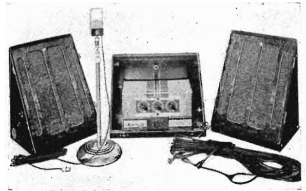
RCA Portable Sound System PG-114
