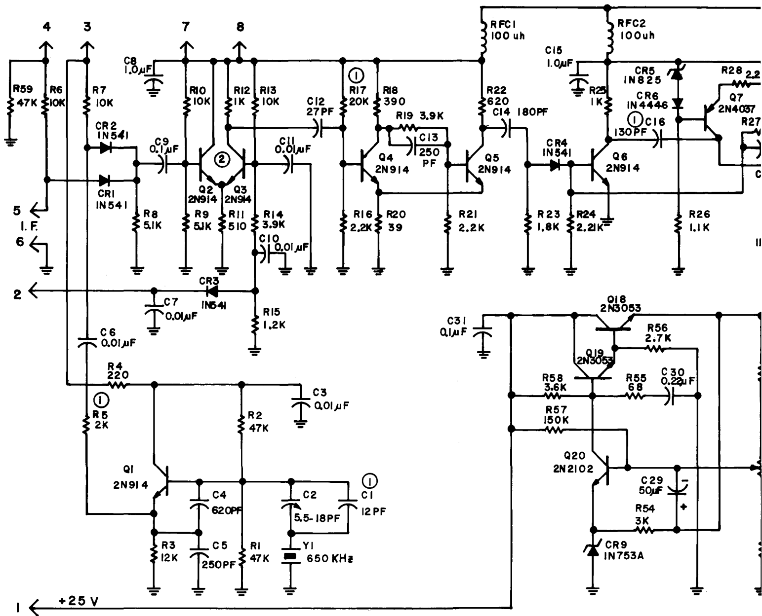
CALIBRATING OSCILLATOR
