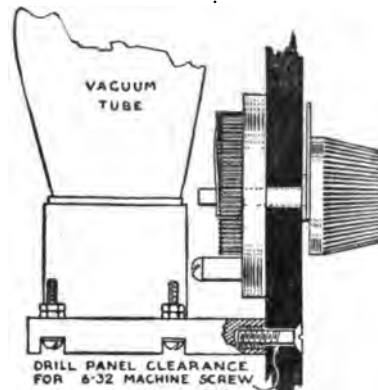
RHEOSTAT AND SOCKET ASSEMBLY
