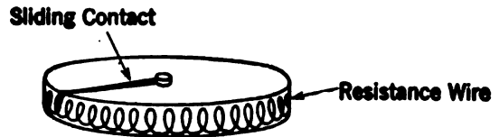
Fig. 4. This is a very popular form of rheostat. The shaft to which the sliding contact is connected is generally made long enough to carry the usual control knob as well as to permit either front or rear of panel mounting. A rheostat of this type permits accurate adjustment of the filament temperature
