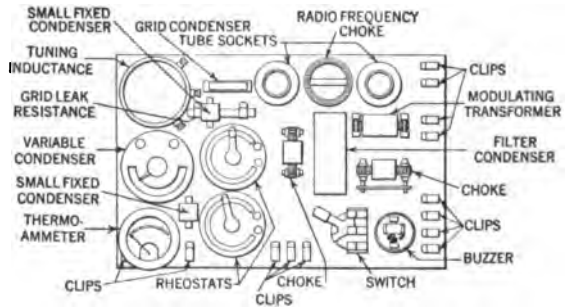
A DISPLAY OF STANDARD RADIO PARTS Assembled, wired and displayed by a progressive radio dealer—a great help to the buying public
