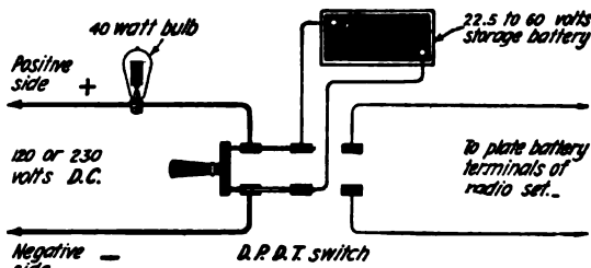
FIG. 6 Charging from a direct current supply
