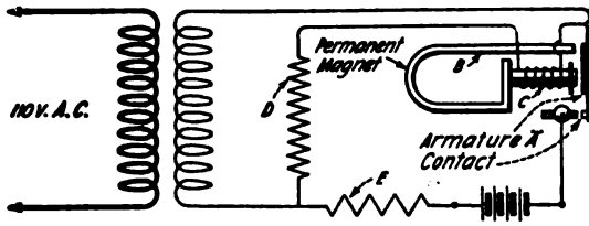
FIG. 17 Another form of vibrating charger
