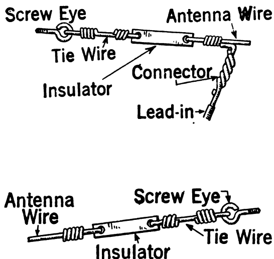
Fig. 6. Details of antenna construction
