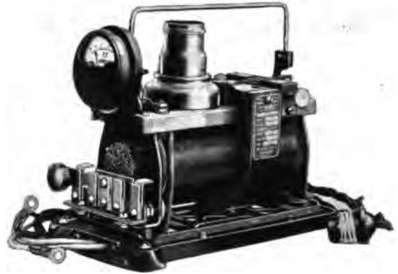
FIG. 19 A vibrating rectifier with switch for charging at different rates
