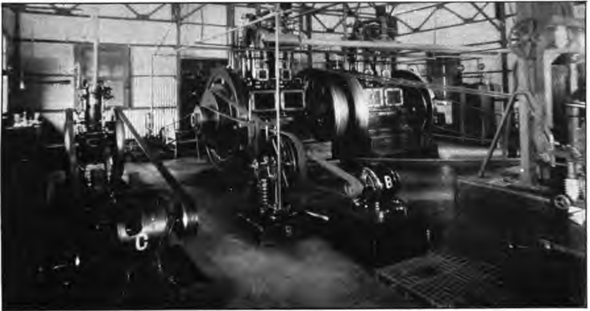
THE 100 H. P. RADIO STATION AT SANTA MARTA, COLOMBIA This view of the power house shows two 50-H. P. kerosene oil engines, air compressor, exciter, a small radio set for ship work, and other machinery
