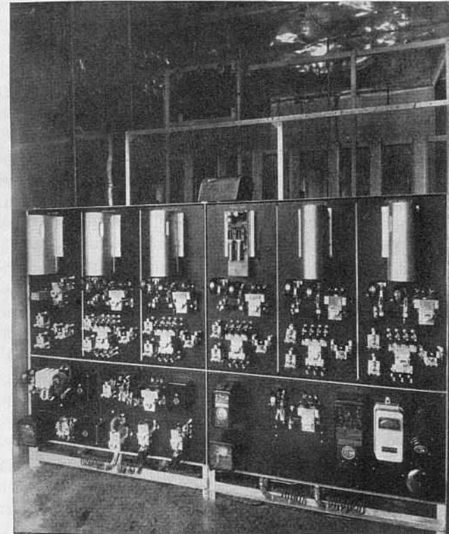
Fig. 13—Control relay panel.
