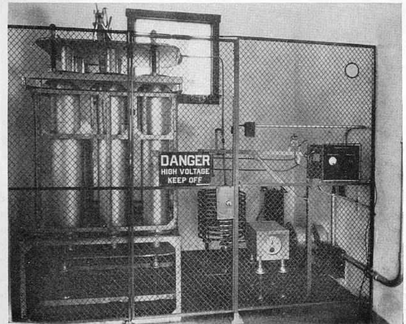
Fig. 9—Antenna tuning house equipment.
