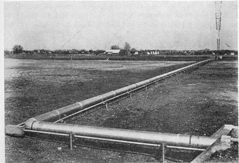
Fig. 8—Seven hundred and eighty foot concentric tube transmission line.
