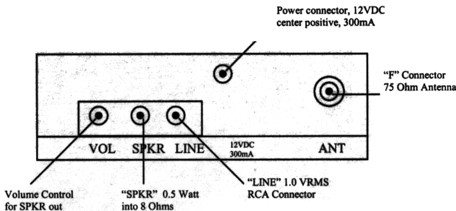
AF 610 REAR PANEL (Individual Unit Chassis or as mounted in the AFC3 chassis)
