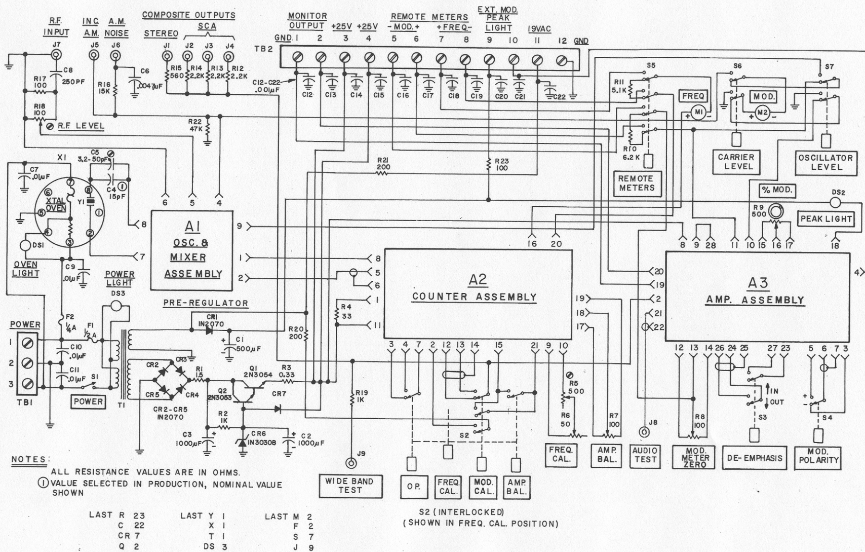
Figure 7-4. FMM-1 Frequency and Modulation Monitor Chassis, Schematic
