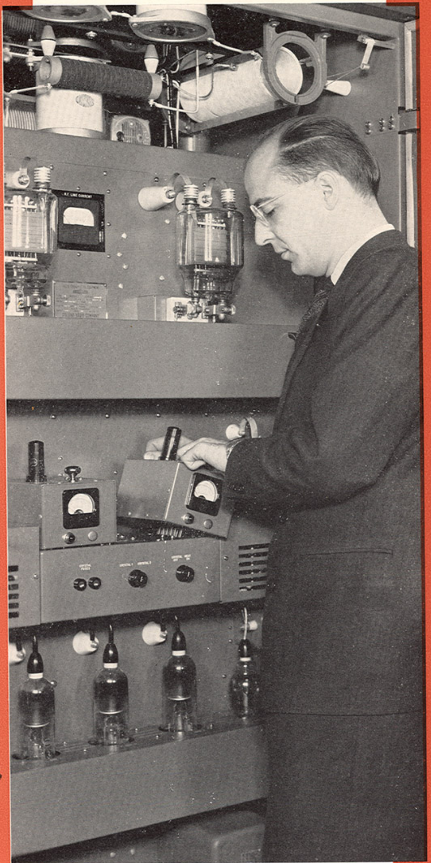
Either oscillator unit can be removed quickly. The selector switch is set to the second unit and transmitter operation continued while the removed oscillator is checked.
