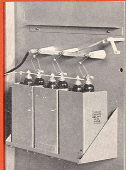
Circuit protection is a major feature of the 20T. All high voltage capacitors are individually fused through a spring connection. If the fuse opens, the spring immediately shorts out the capacitor and isolates it from the circuit.
