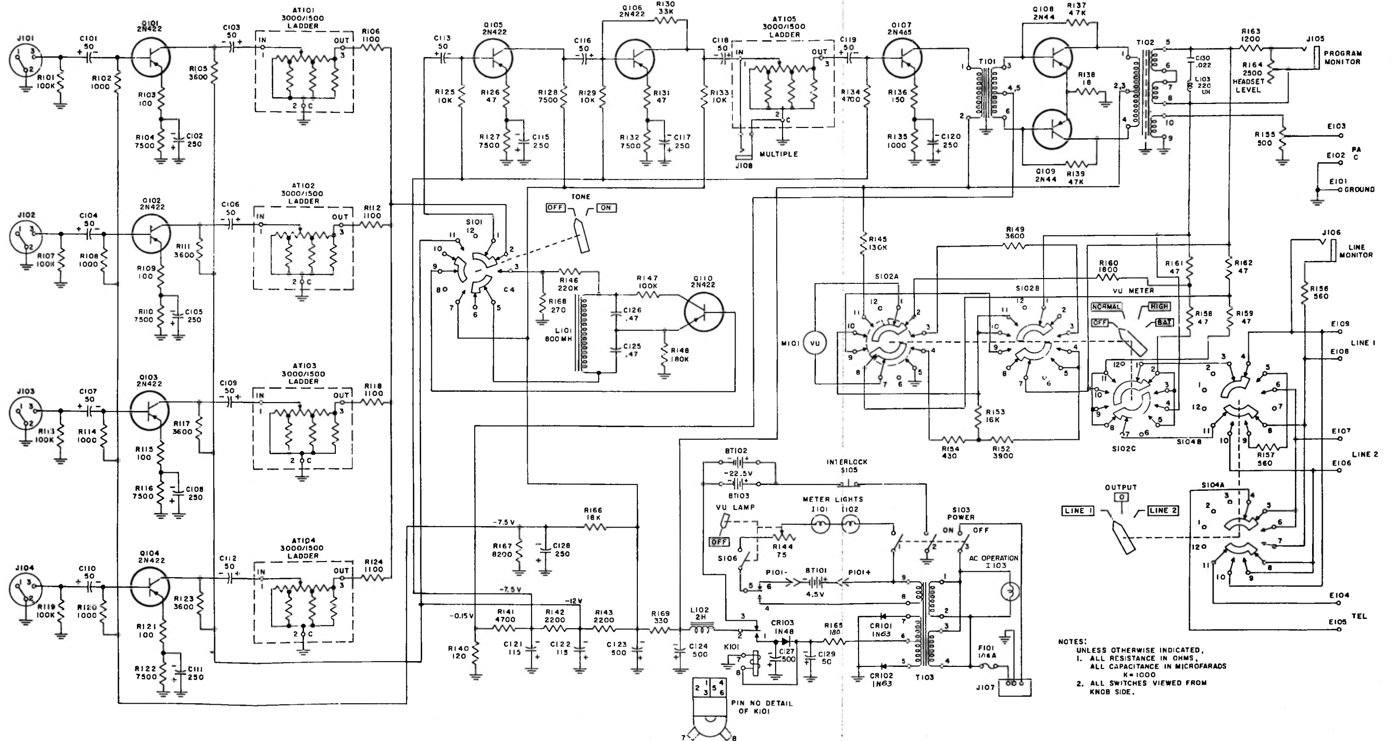
Figure 7-5. 212Z-1 Remote Amplifier, Complete Schematic
