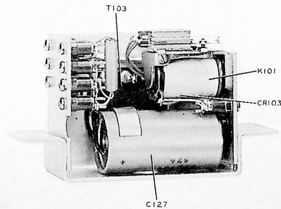
Figure 7-4. Power Supply, Side Open View
