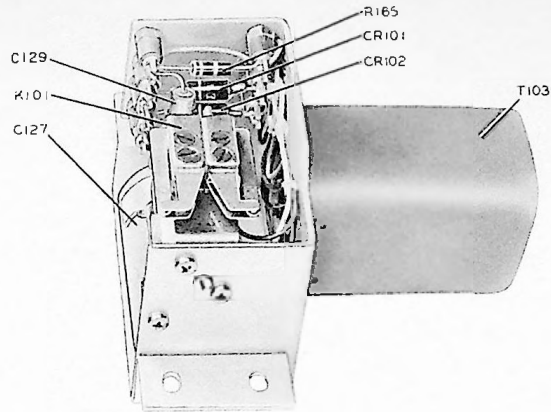
Figure 7-3. Power Supply, Top Open View
