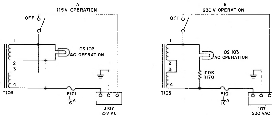
Figure 2-2. 115V/230V Input Power Change, Schematic Diagram
