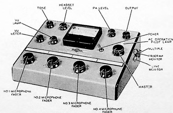
Figure 3-1. 212Z-1 Remote Amplifier, Controls
