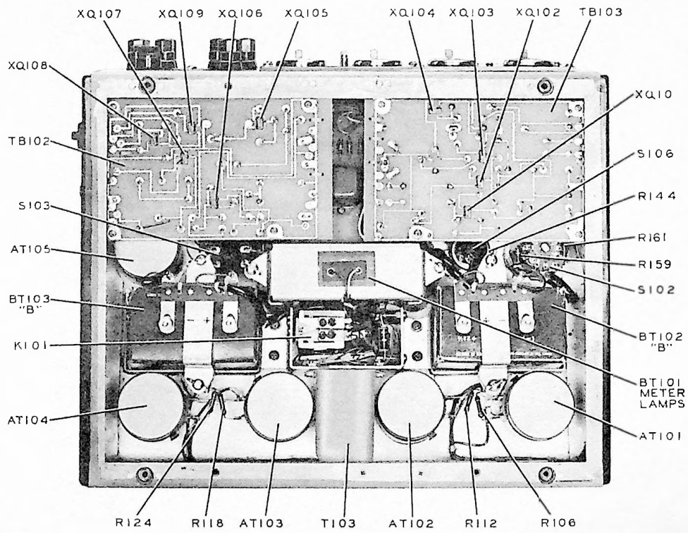
Figure 7-1. 212Z-1 Remote Amplifier, Bottom View
