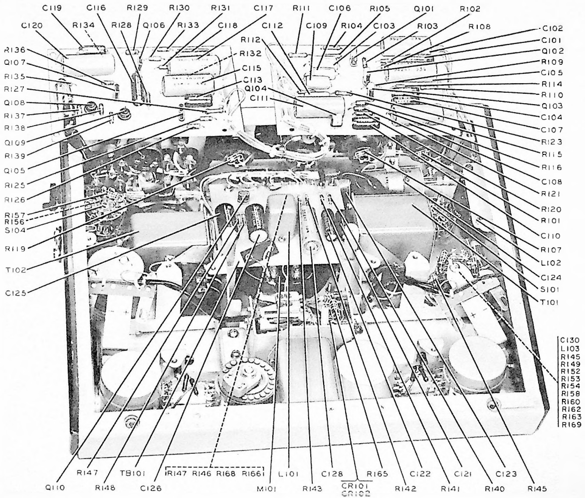
Figure 7-2. 212Z-1 Remote Amplifier, Bottom Open, Boards Removed
