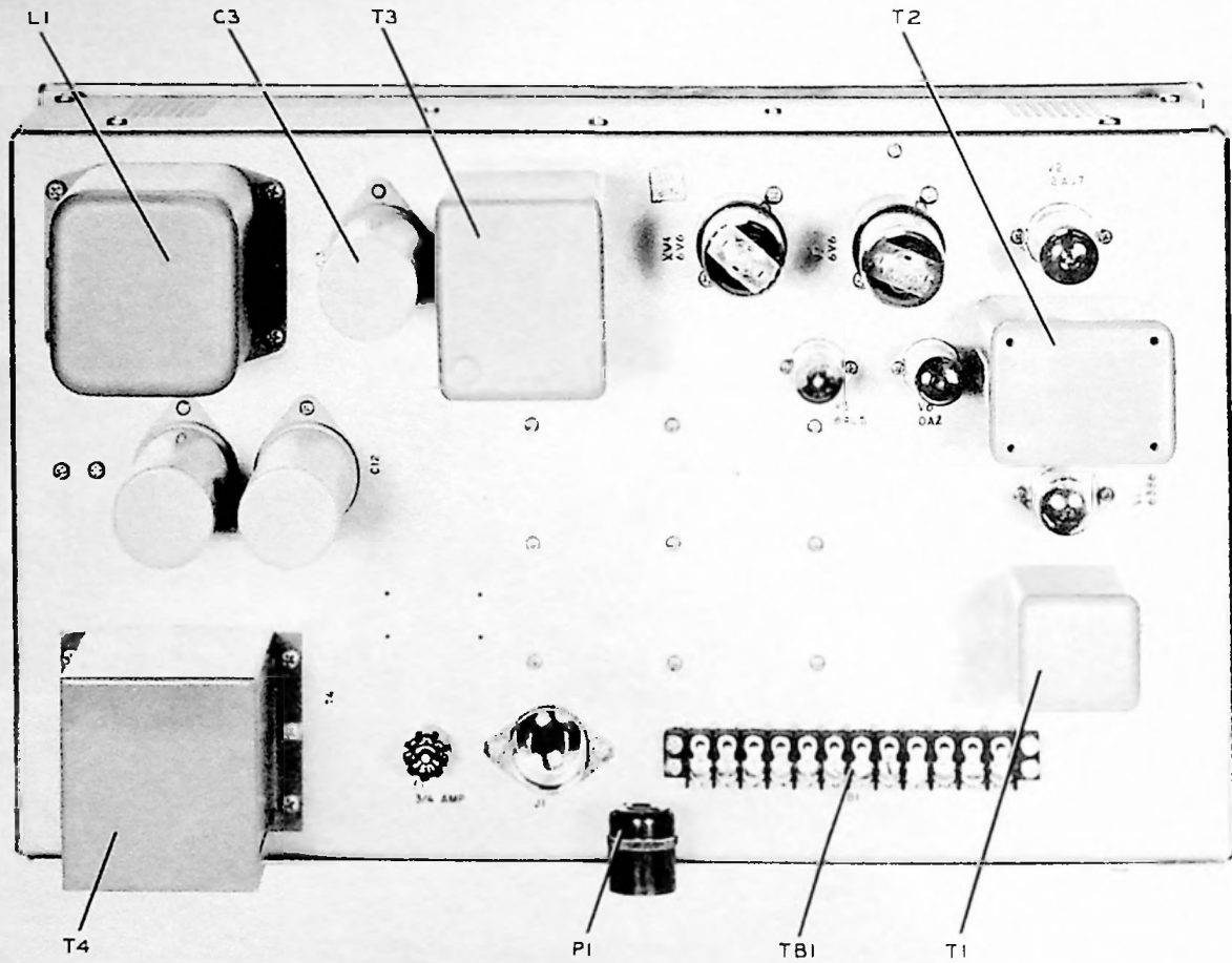
Figure 6-4. Peak Limiting Amplifier 26U-1, Rear View
