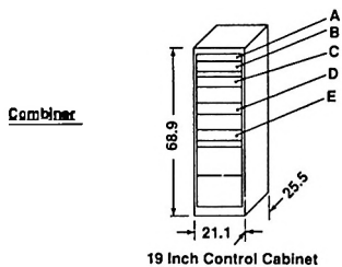
Typical Set-up: 70 kW FM Transmitters
