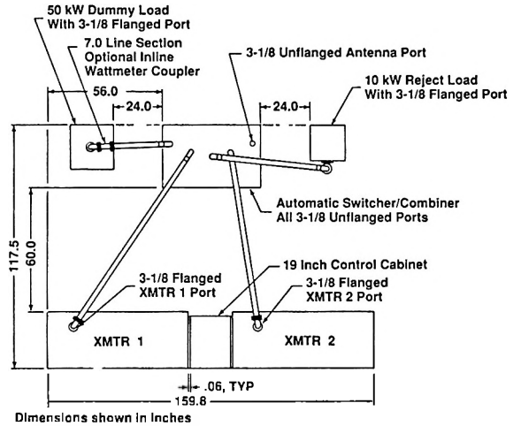
Typical Plan View, 40 kW FM Transmitters
