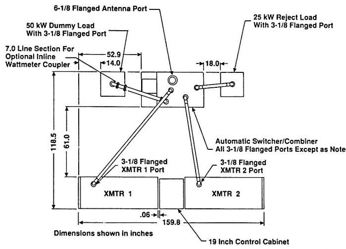
Typical Plan View, 50 & 55 kW FM Transmitters
