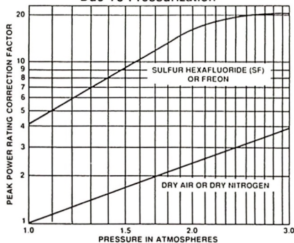
Peak Power Rating Improvement Due To Pressurization
