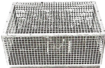
Type 516DL-1, 5,000/10,000 watt Dummy Load
