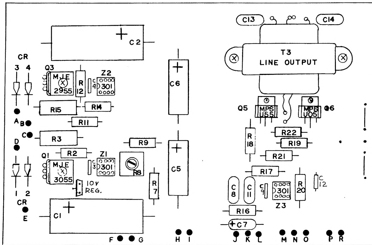
POWER SUPPLY/LINE AMPLIFIER PC ASSEMBLY
