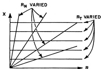
Figure 6. Loci of R_n and R_t Adjustments on Z Plane.
