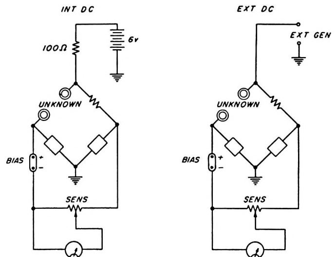
Figure 5. Source and Detector Diagrams.
