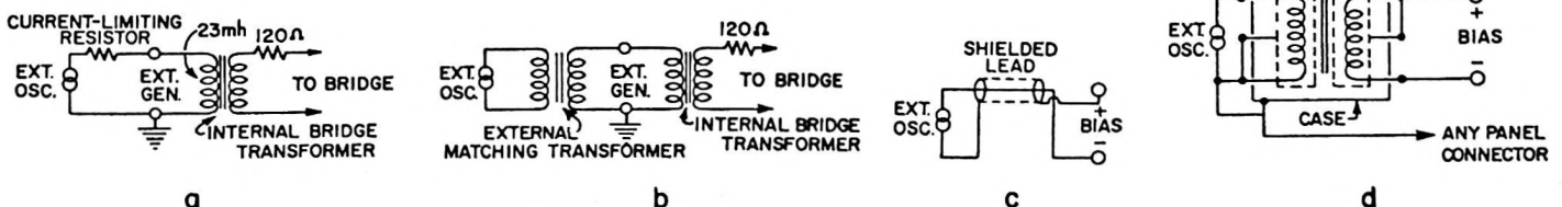
Figure 13. Methods of Applying External AC.
