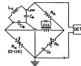
Figure 12. Capacitance to Ground for Inductance Measurement.
