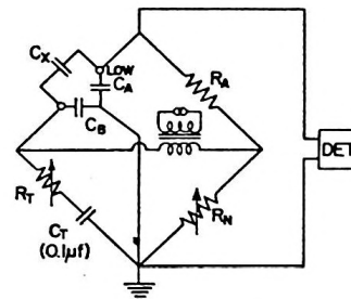
Figure 11. Capacitance to Ground for Capacitance Measurement.
