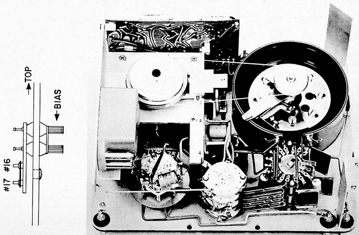
Figure 21. Rear Interior View.
