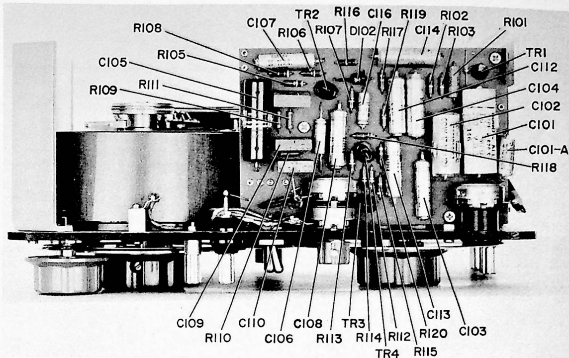
Figure 20. Bottom Interior View.
