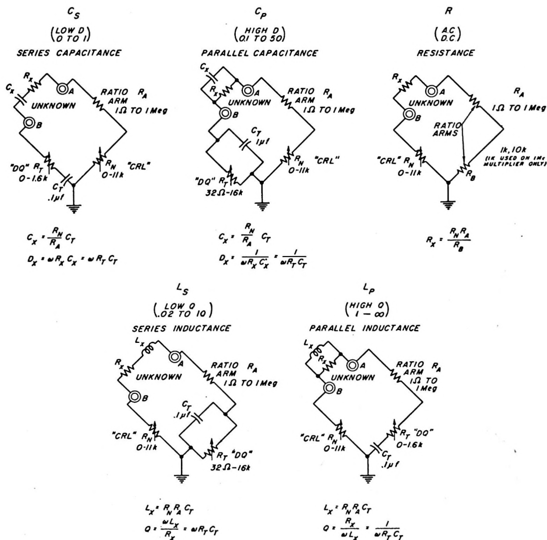
Figure 3. Bridge Circuits Used in Impedance Bridge.
