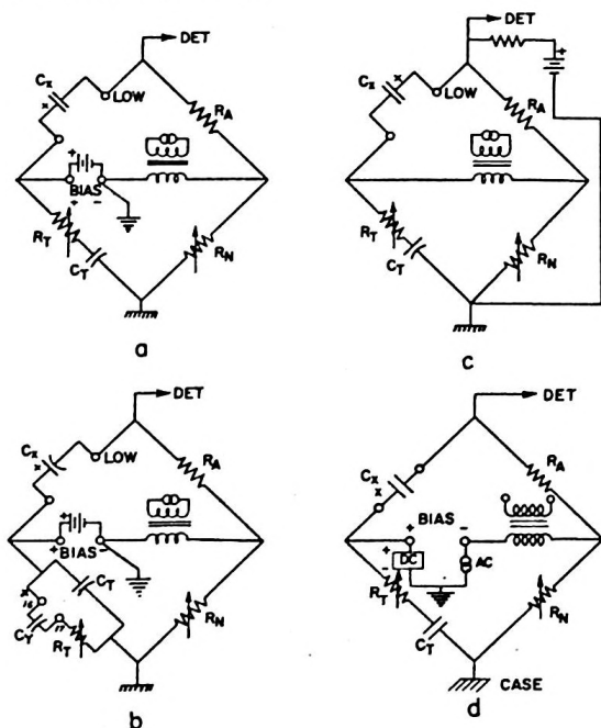
Figure 15. Methods of Applying DC Voltages to Capacitors.
