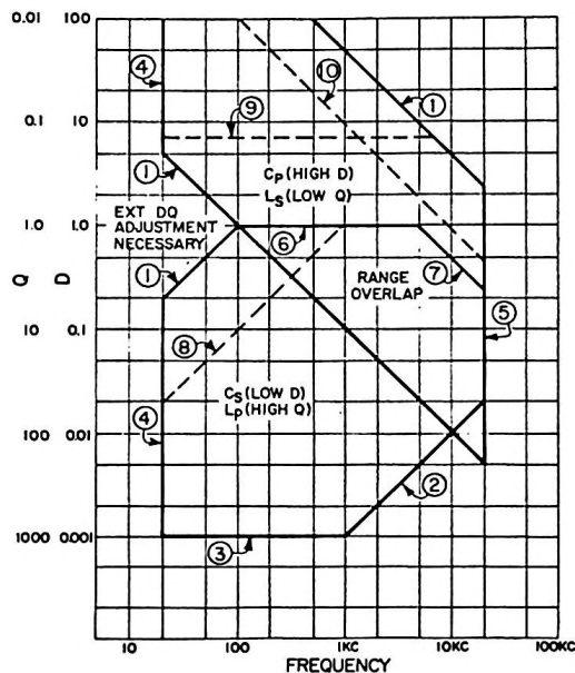
Figure 14. DQ Ranges vs Frequency. (Refer to paragraph 6.4.)
