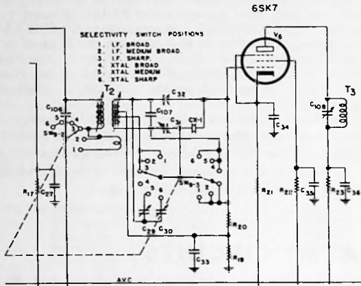
FIG. 2—CRYSTAL FILTER SCHEMATIC
