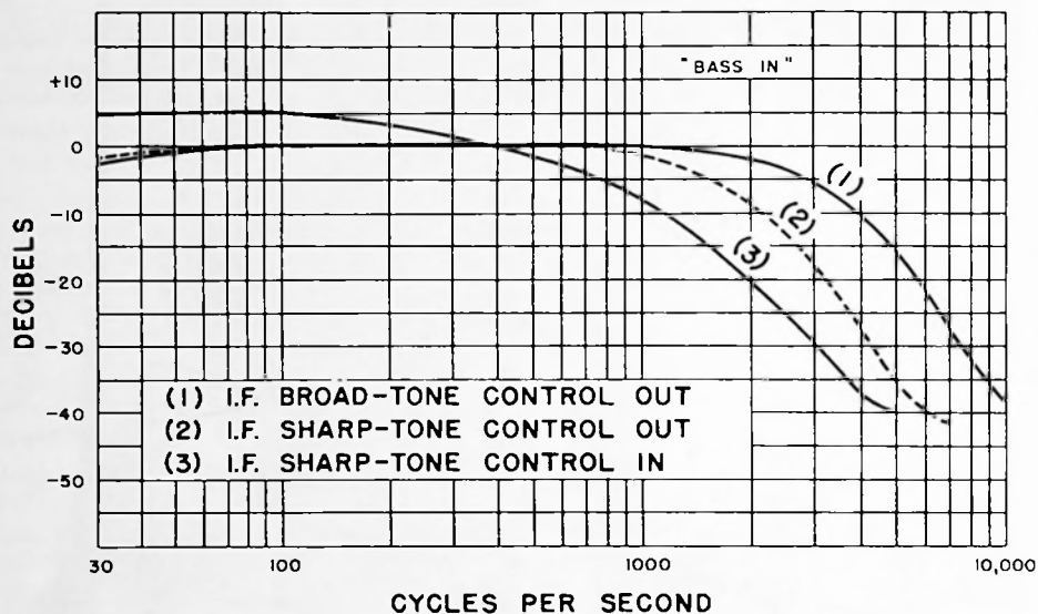
FIG. 10—AUDIO FIDELITY CURVE
