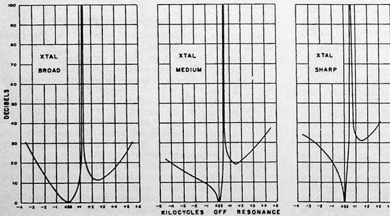
FIG. 4—CRYSTAL SELECTIVITY
