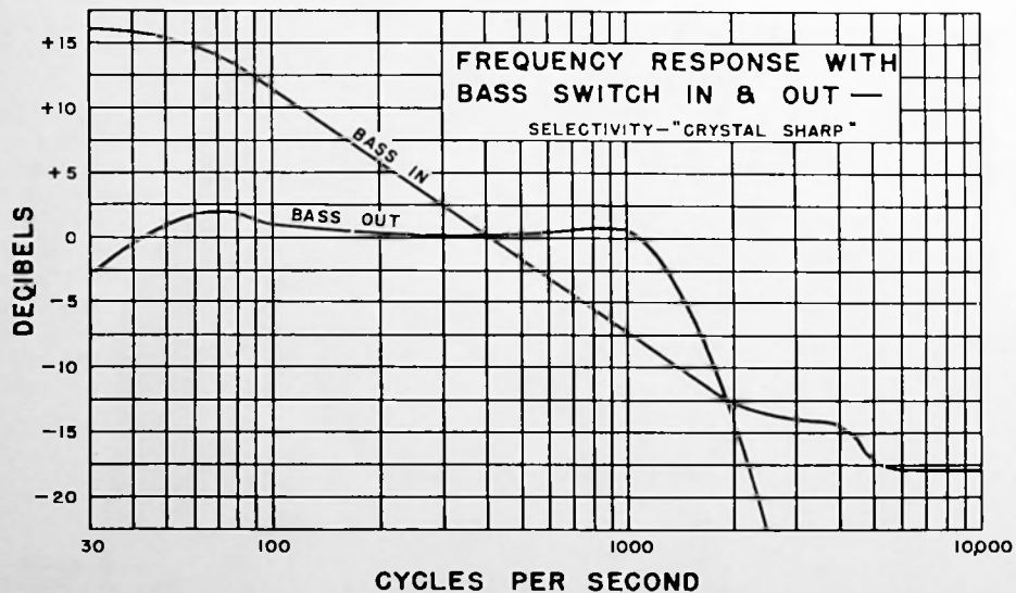
FIG. 11—AUDIO FILTER CURVE
