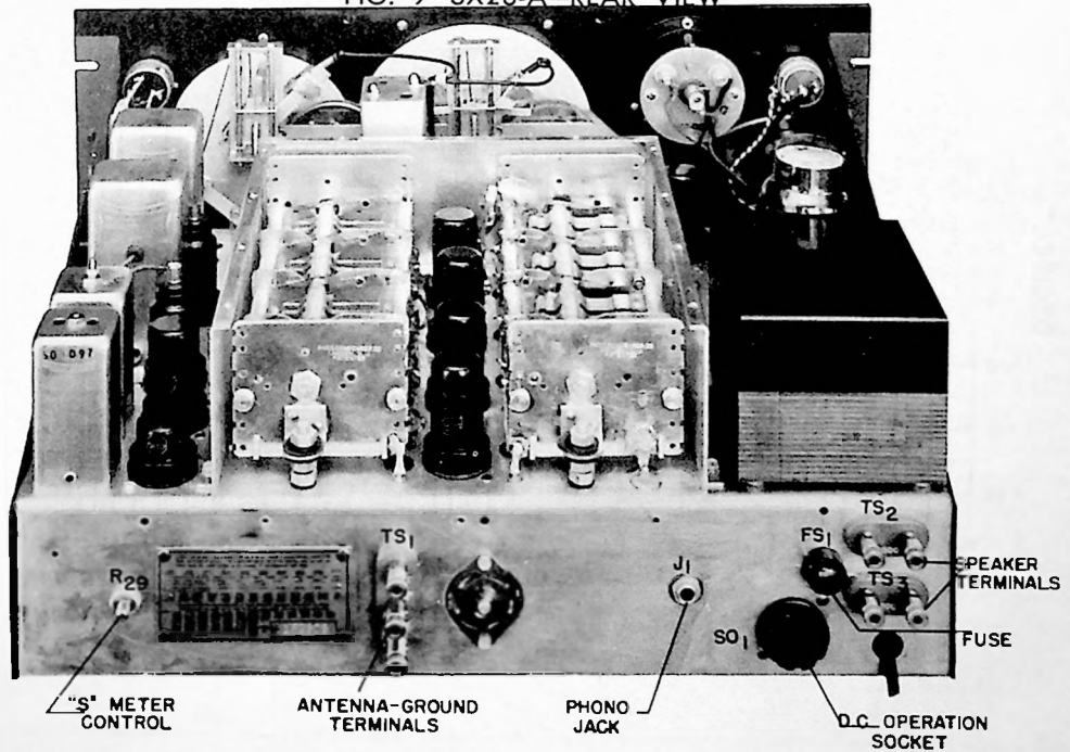
FIG. 9—SX28-A—REAR VIEW
