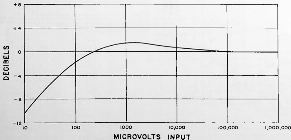
FIG. 7—A.V.C. CURVE—AT 3 MC.
