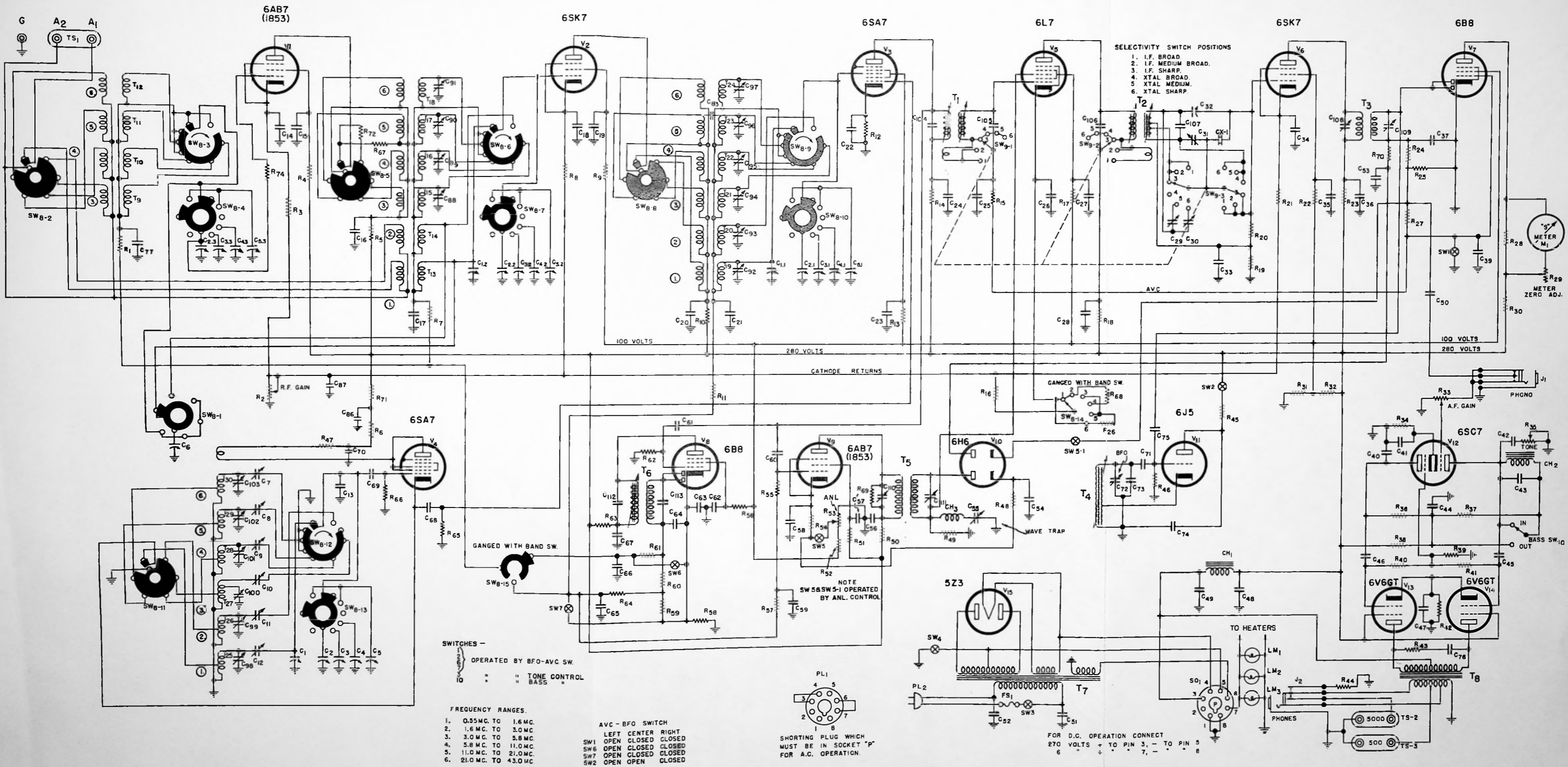
FIG. 13-SX28-A-SCHEMATIC
