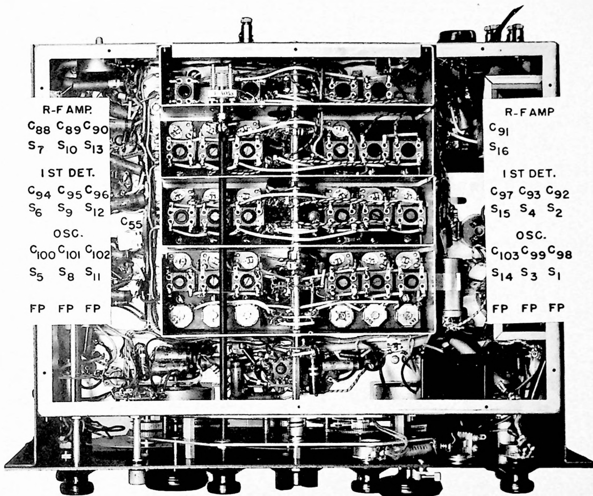
FIG. 12—RF AND OSC ADJUSTMENT LOCATION AND ALIGNMENT PROCEDURE
