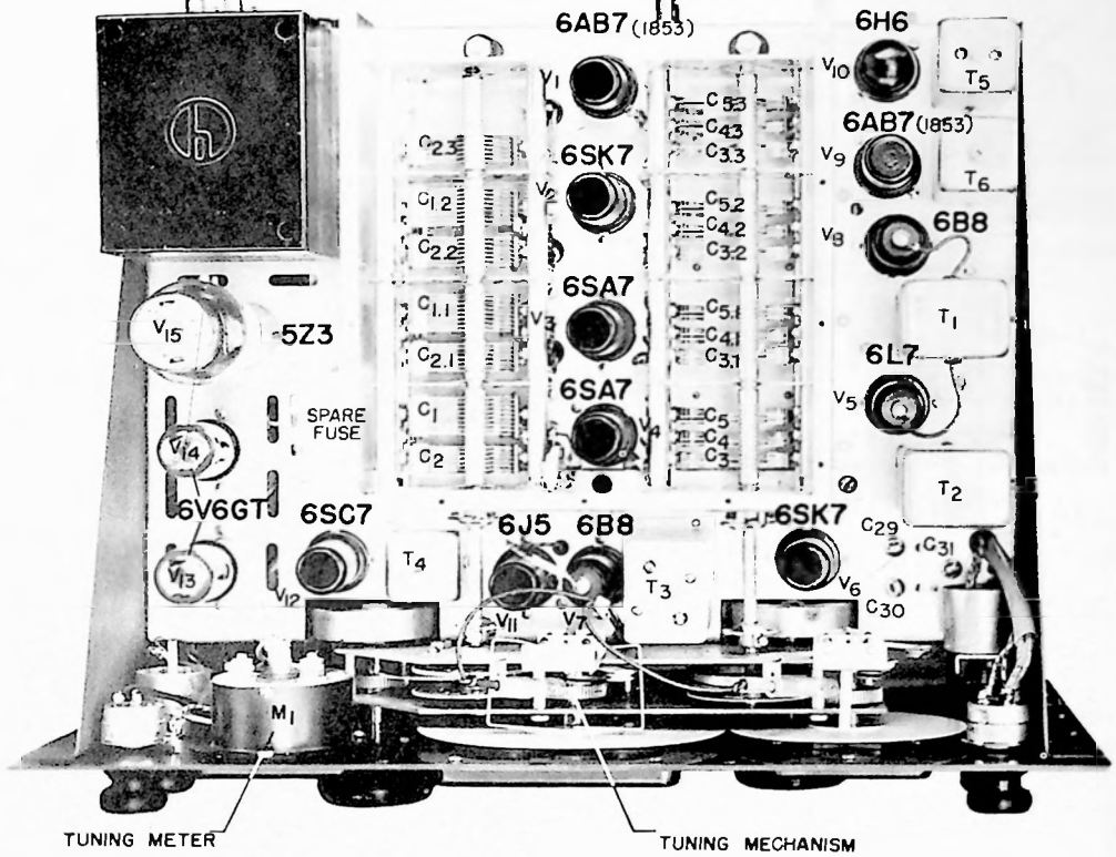
FIG. 9—SX28-A—REAR VIEW
