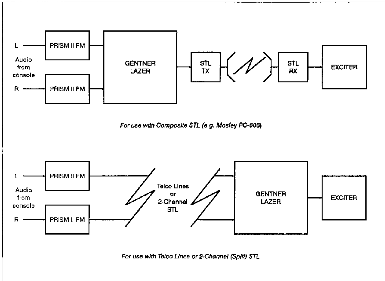
Figure 2-1 Recommended FM Configurations
