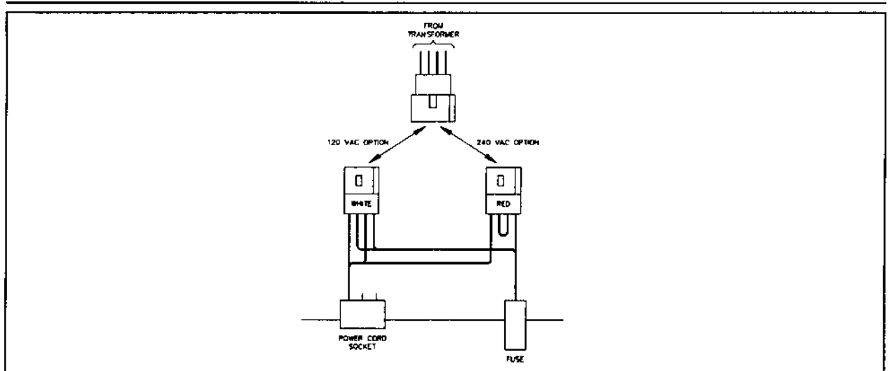
Figure 2-6 AC Power Wiring Harness
