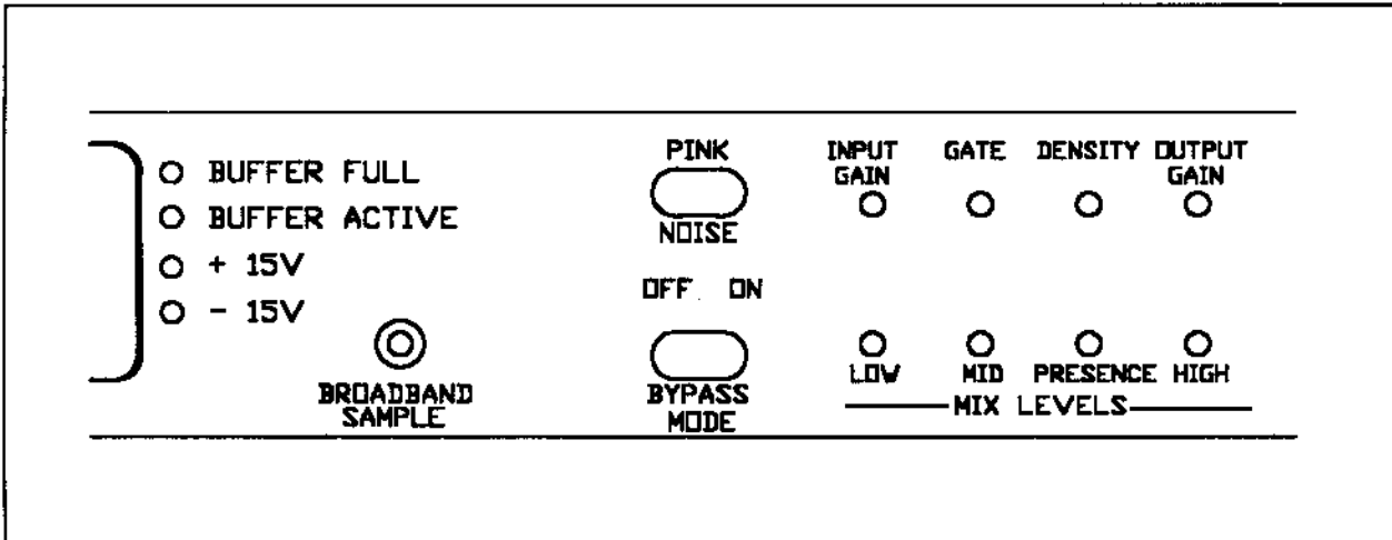
Figure 2-5 PRISM II FM Control Panel
