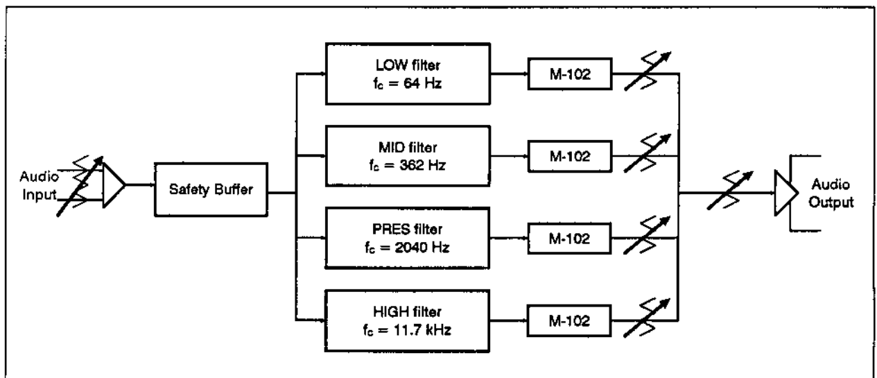
Figure 2-2 PRISM II FM Block Diagram
