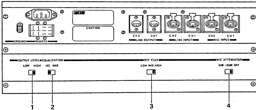
Fig. 2-2(b) Standard Switch Position on Shipment (IEC)
