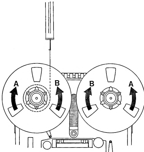
Fig. 6-2 Brake Measurement
