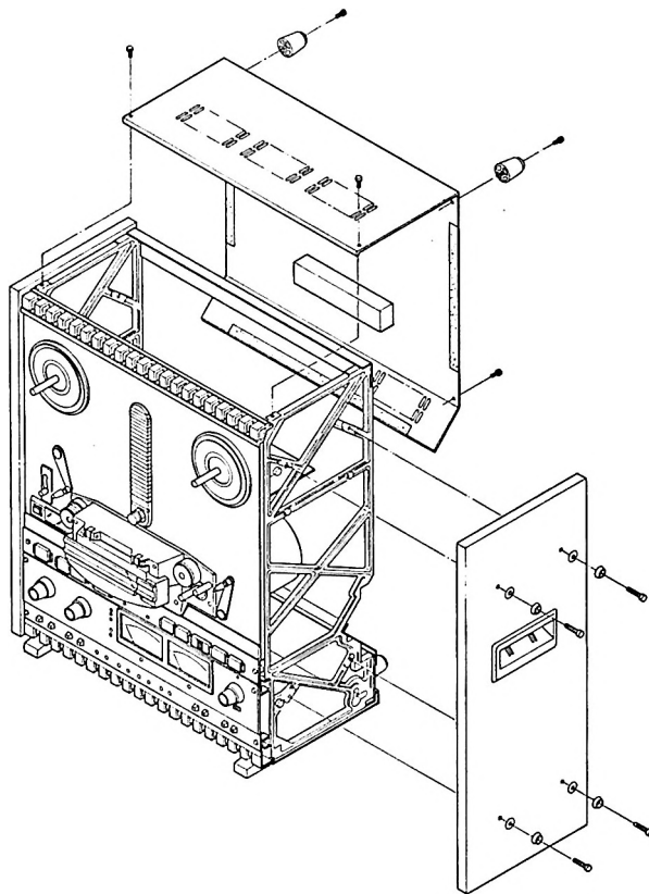
Fig. 6-1 Rear Panel and Side Board Removal
