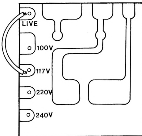
Fig. 2-3 Voltage Selection Terminal
