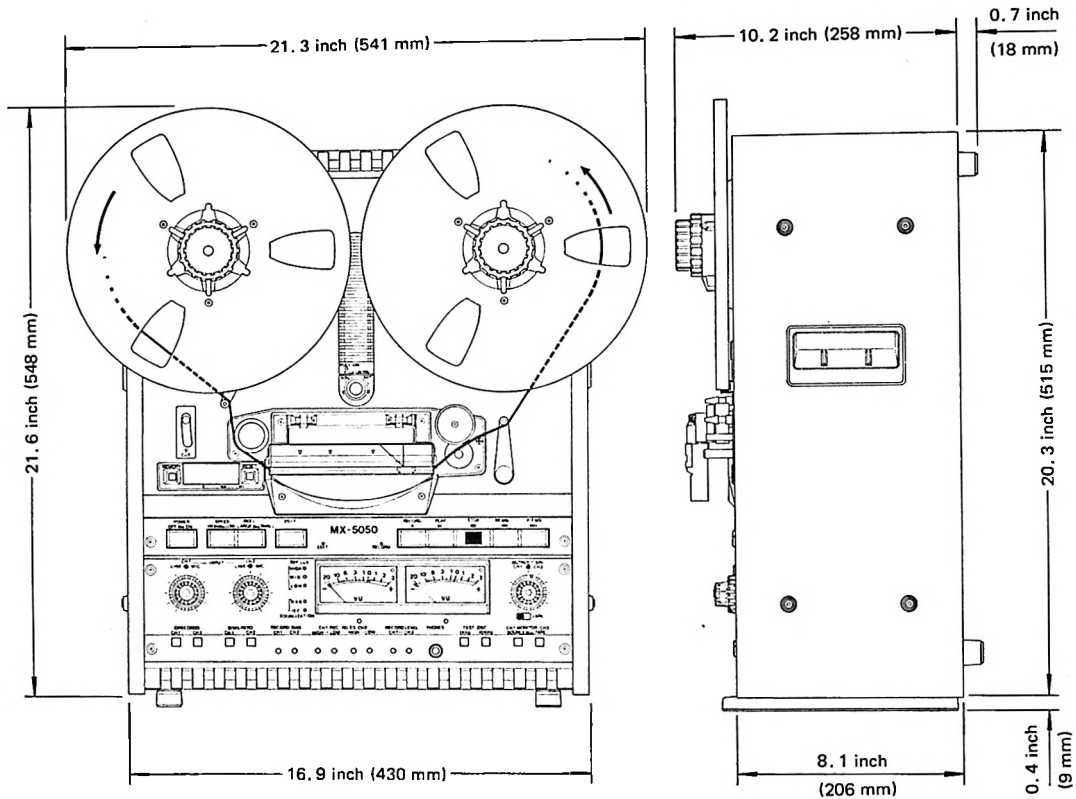
Fig. 2-1 Equipment Dimensions
