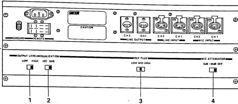
Fig. 2-2(a) Standard Switch Position on Shipment (NAB)
