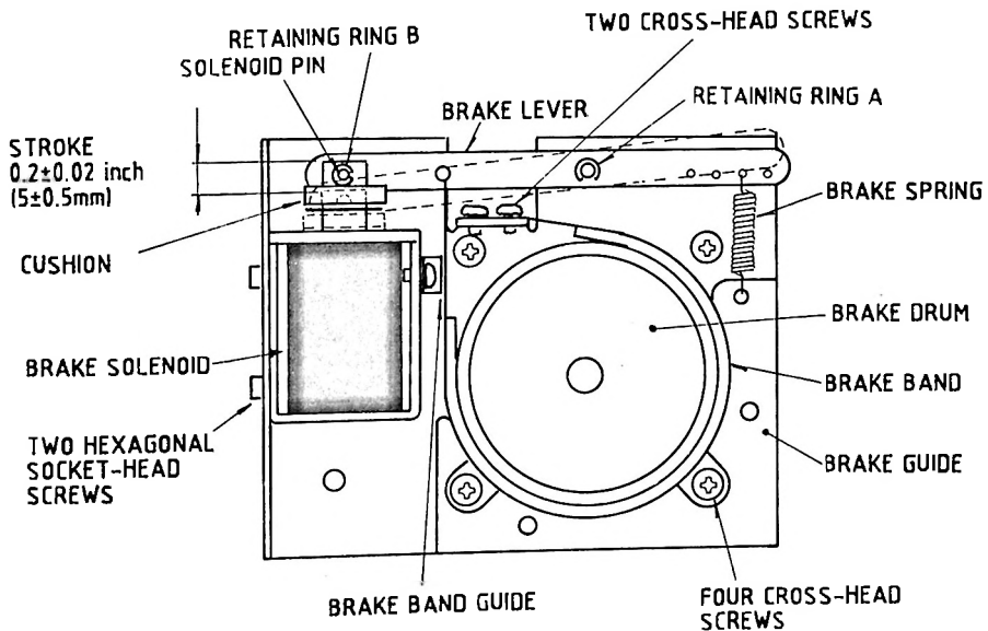
Fig. 6-3 Brake Assembly Location
