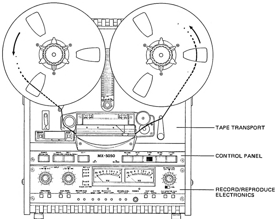
Fig. 1-1 MX-5050BII Major Components
