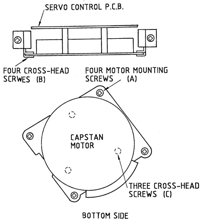
Fig. 6-10 Location of DC Servo Capstan Motor
