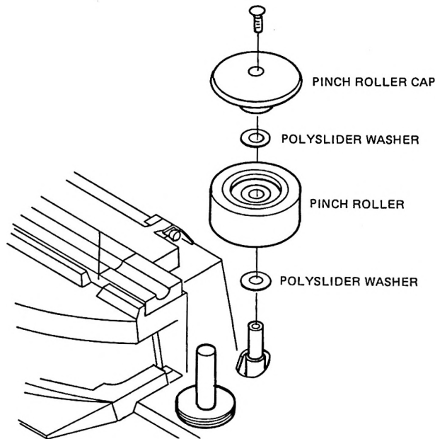
Fig. 6-11 Pinch Roller Removal
