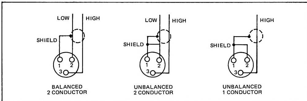
Fig. 2-4 Input/Output Assembly Connector Wiring
