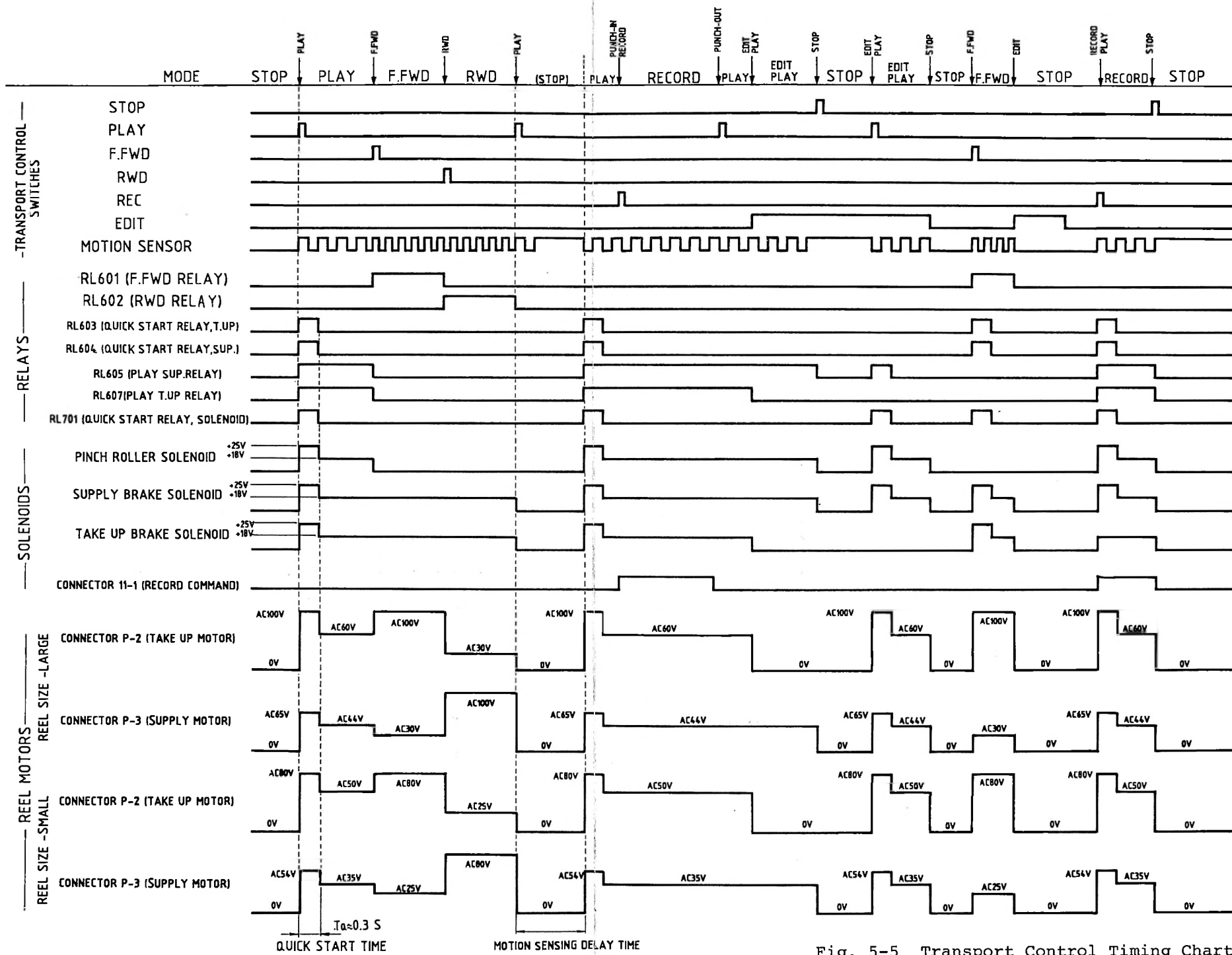
Fig. 5-5 Transport Control Timing Chart
