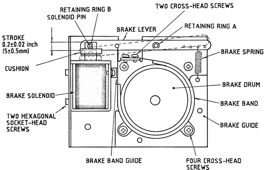
Fig. 6-9 Brake Assembly
