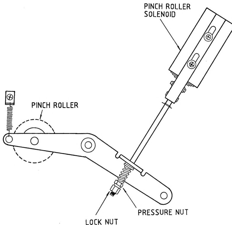
Fig. 6-5 Pinch Roller Pressure Adjustment
