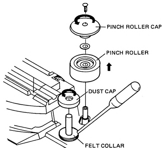
Fig. 4-3 Lubrication
