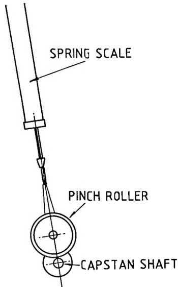
Fig. 6-4 Pinch Roller Pressure Measurement
