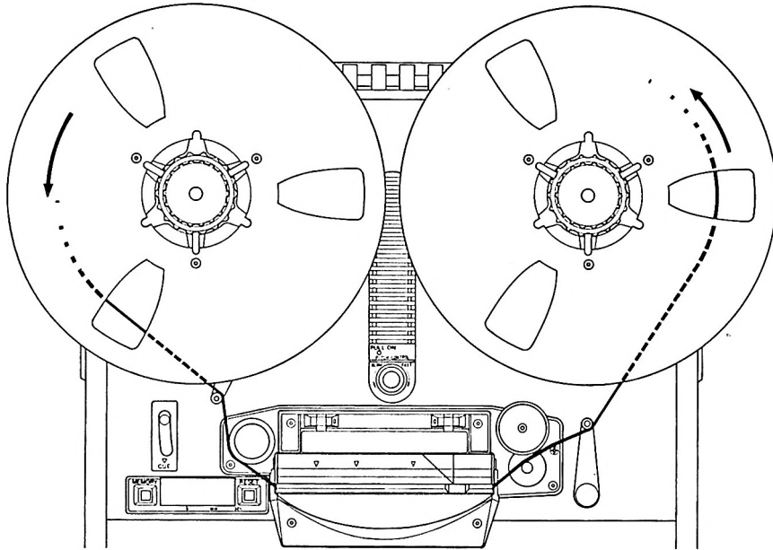
Fig. 3-2 Tape Threading
