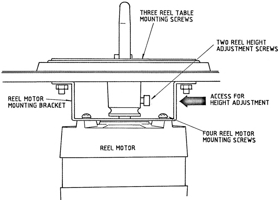
Fig. 6-8 Reel Motor Mounting
