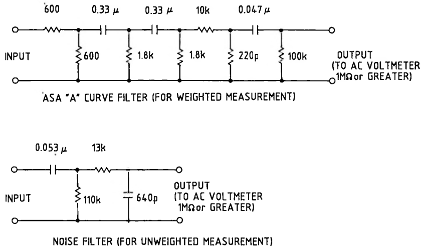
Fig. 7-1 Filter Schematics
