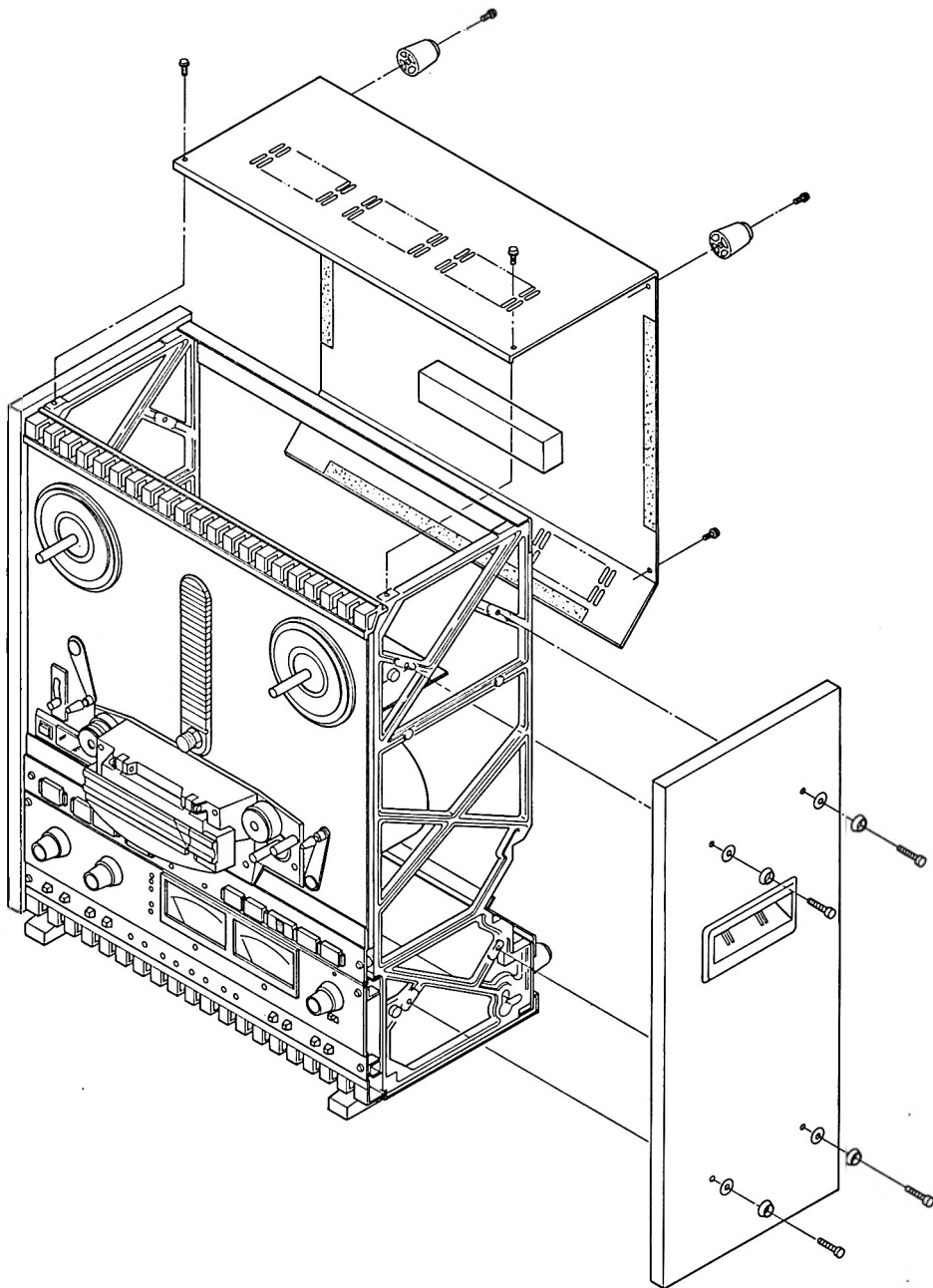
Fig. 5-2 Rear Panel and Side Board Removal
