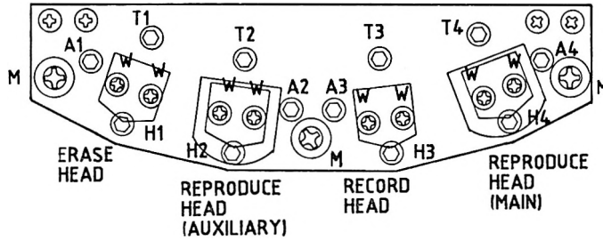
Fig. 6-12 Head Assembly
