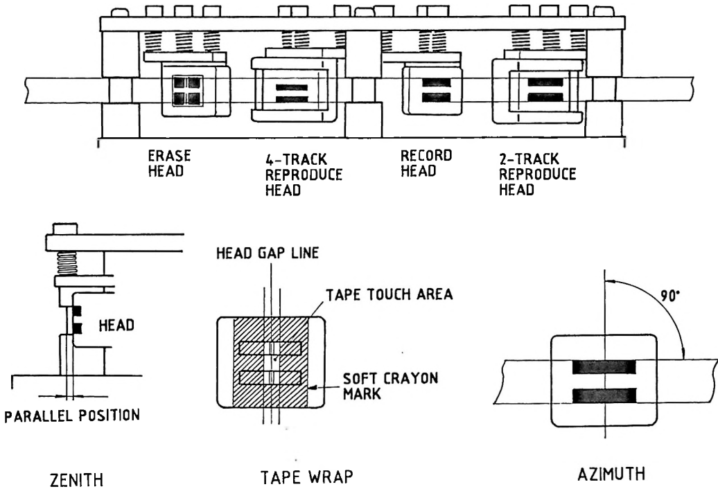
Fig. 6-13 Head Alignment
