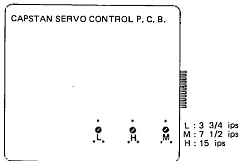
Fig. 6-7 Capstan Servo Control P.C.B.
