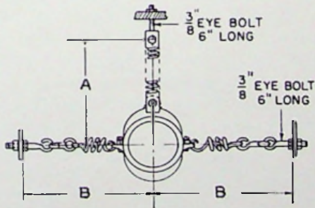
(3-POINT HANGER, SINGLE)
