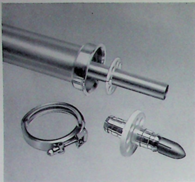
Close up view of RCA Universal Transmission Line with Marman Clamp and Inner Connector
