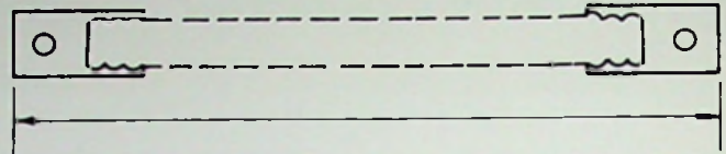
Drawing showing points of measurement used in spring pre-loading tables for RCA expansion hangers. Charts give length in inches.
