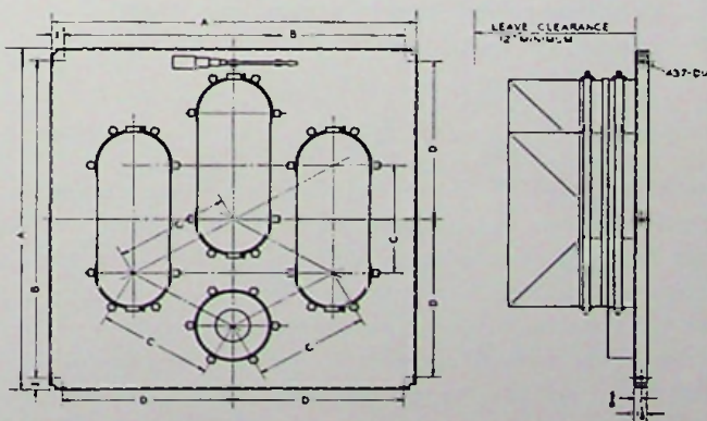
Outline Dimensions, 3-Pole Panels
