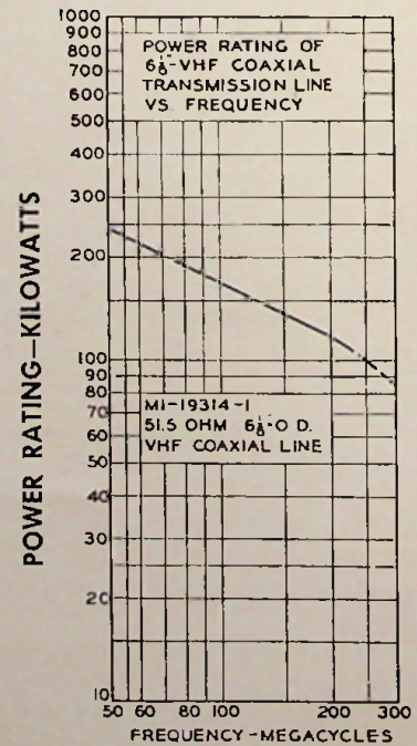
POWER RATING—6 1/8" LINE
