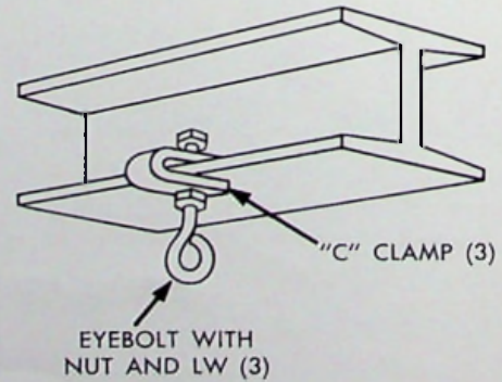
MI-27705 FOR 3/8" & 6/8"
