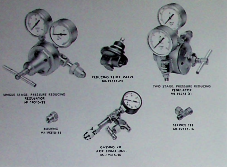
Precision gauges and accessories for gassed systems.
