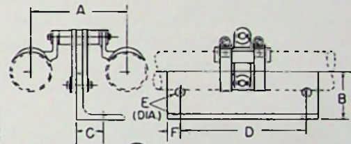
(SWIVEL HANGERS)
