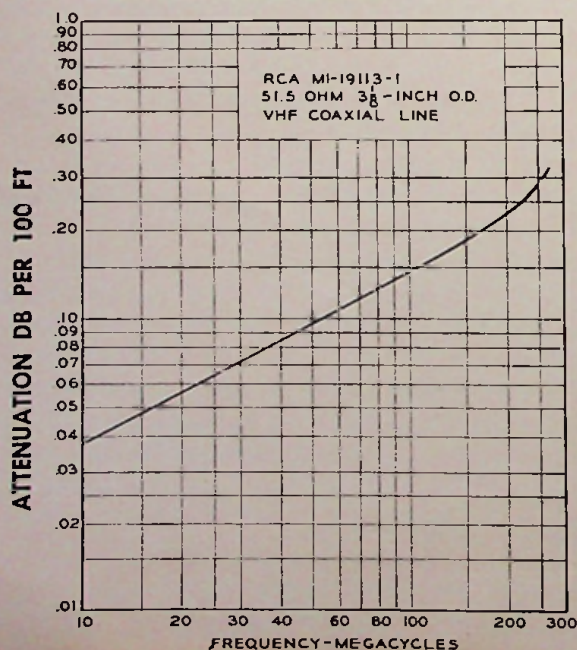
ATTENUATION—3 1/8" LINE
