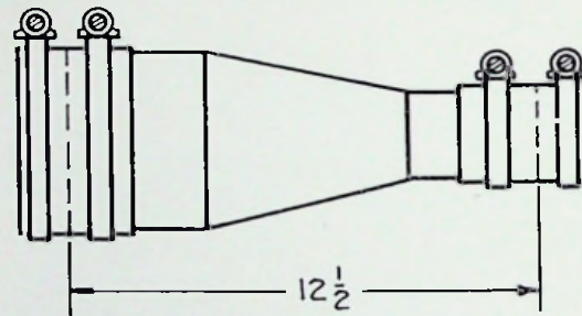
REDUCER (UNGASSED) 6 1/8-3 1/8 MI-19314-C-13
