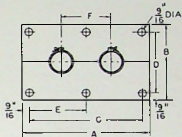
(HORIZONTAL ANCHOR, DUAL)
