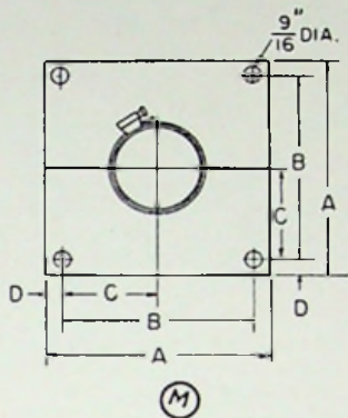
(HORIZONTAL ANCHOR, SINGLE)
