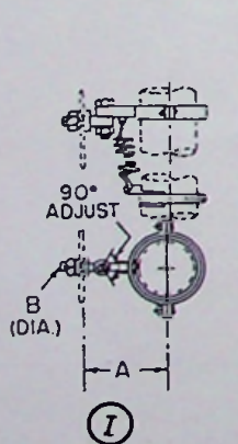
(WITH PIVOT. MOUNT THROUGH HOLE)
