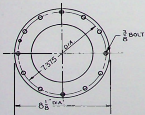
FIXED FLANGE MI-19314-C-11 OR SWIVEL FLANGE MI-19314-C-12
