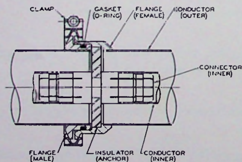
Cut-away drawing showing flanged connector assembly of Transmission Line.
