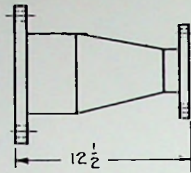
REDUCER (GASSED) 6 1/8-3 1/8 MI-19314-C-4
