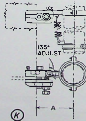
(WITH PIVOT. CLAMP ON FLAT MEMBERS)
