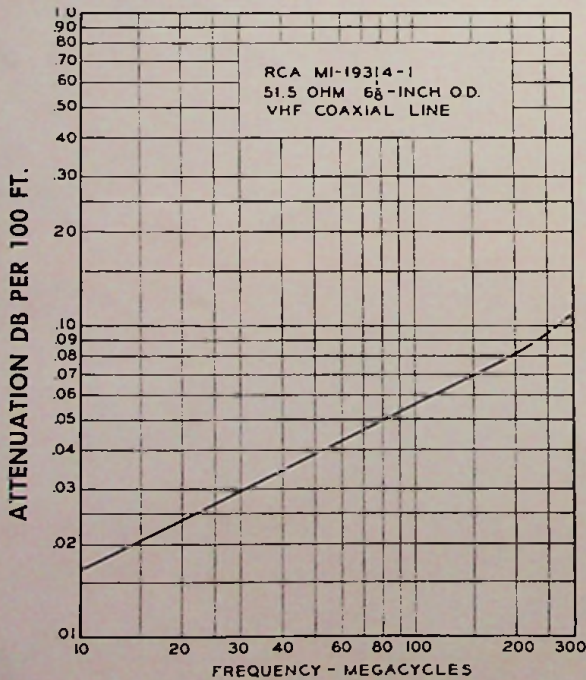
ATTENUATION—6 1/8" LINE
