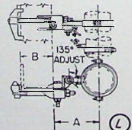
(WITH PIVOT. CLAMP ON ANGLES)
