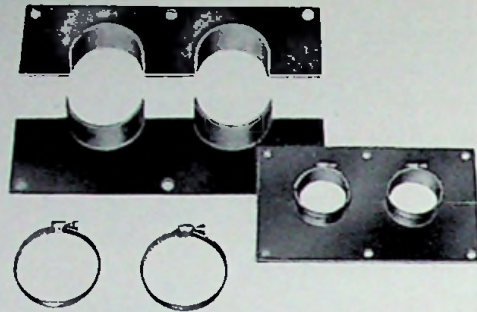
HORIZONTAL ANCHOR FOR SUPPORTING DUAL LINES MI-19312-18-1 \frac{5}{8} MI-19313-18-3 \frac{3}{8} MI-19314-49-6 \frac{1}{8} MI-27900-49-9 \frac{3}{16}
