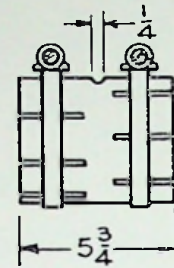
STRAIGHT COUPLING MI-19314-C-7
