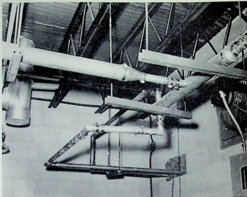
View at rear of transmitter showing typical mounting of diplexer and phasing section utilizing 1½" transmission line for construction of phasing section and 3½" Teflon line in balance of installation.
