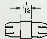
INNER CONNECTOR MI-19314-C-5
