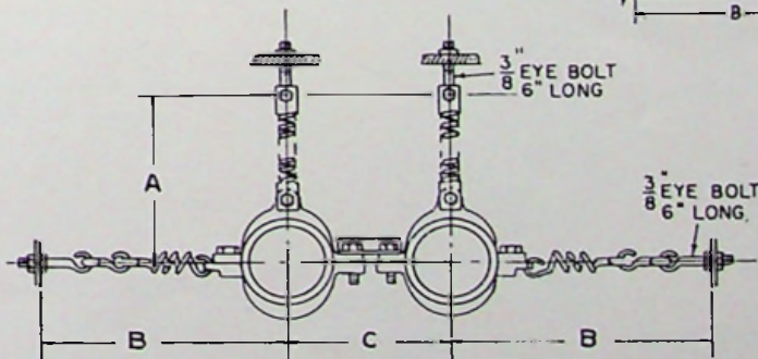
(3-POINT HANGER, DUAL)
