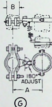
(WITH PIVOT. CLAMP ON ROUND MEMBERS)
