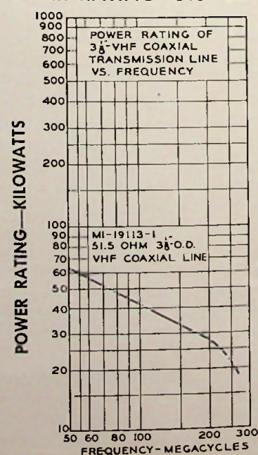
POWER RATING—3 1/8" LINE
