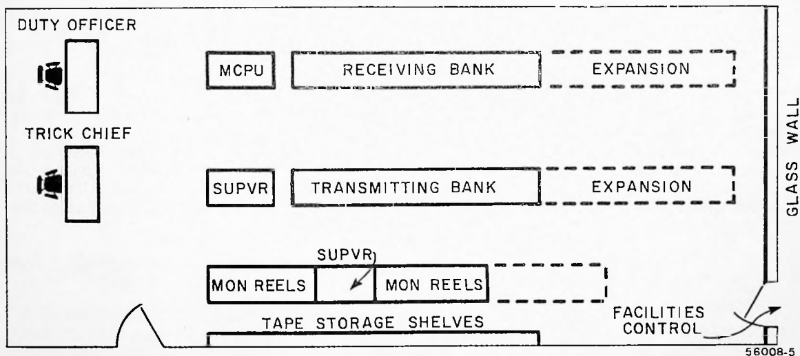
Figure 5. Type tape relay equipment layout for AN/FGC-38 or similar equipment (not to scale).
