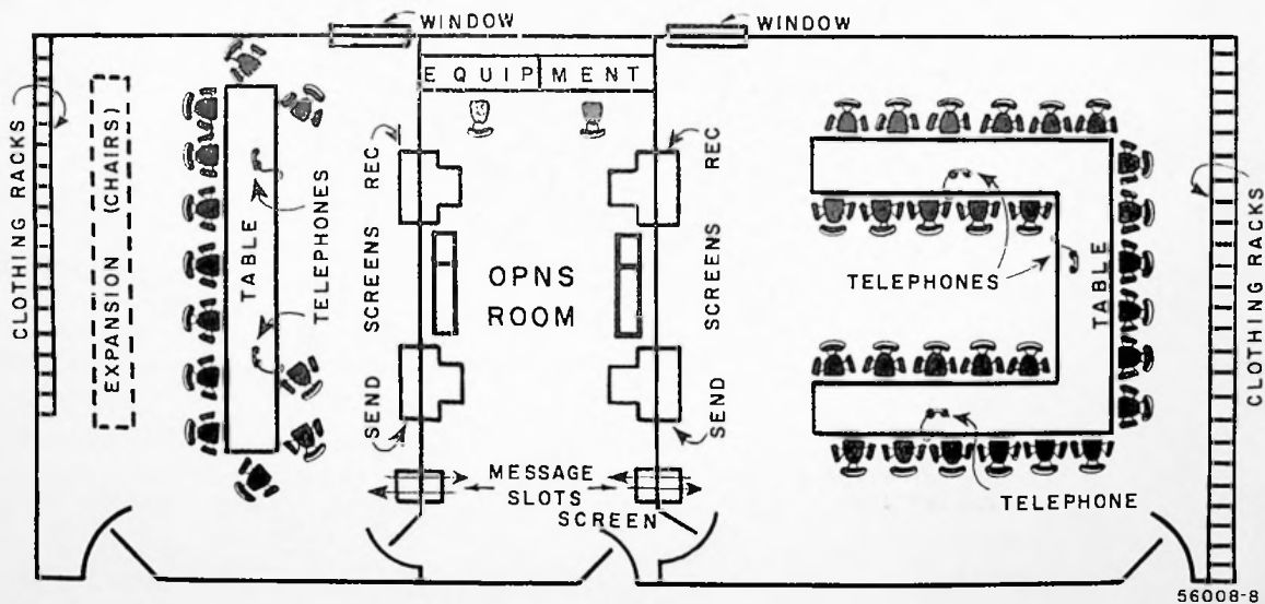
Figure 8. Type TELECON facility - double conference, capacity: 12 seated (Room #2), 18-28 seated (Room #1), plus 10 standees (Room #1) (not to scale).
