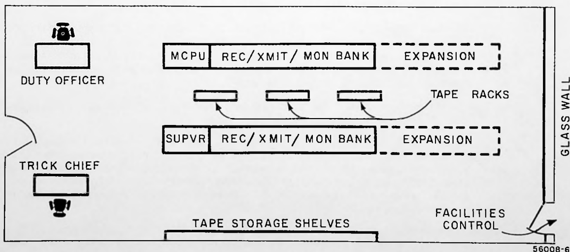
Figure 6. Type tape relay equipment layout for AN/TGC-1 or similar equipment (not to scale).
