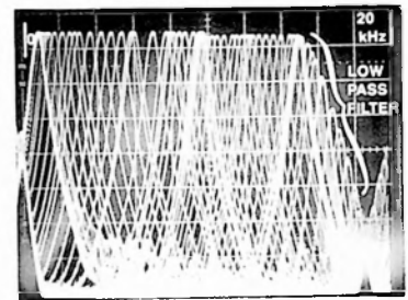
Fig. 20. Checking Audio Response Using Slow Sweep and Storage
