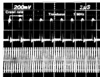
Fig. 40. Oscilloscope Comparison of 5 MHz WWV Against 1 MHz Time Base (figure 40). Adjust counter time base until 10^{-6} accuracy is achieved.
