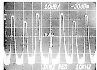
Fig. 43. Indication of the Second Null Using a Spectrum Analyzer
