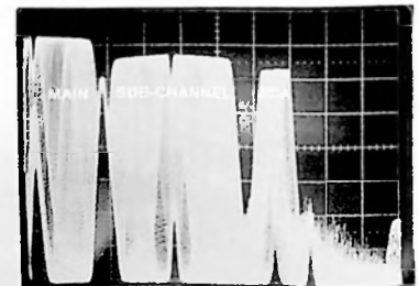
Fig. 6. Composite Fm Stereo Signal Display Obtained by Sweeping with a De-emphasis Filter
