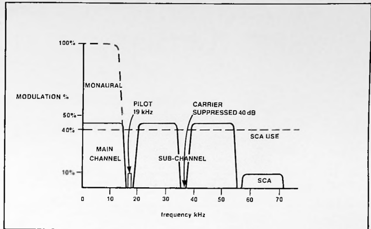
Fig. 1. The Composite Fm Stereo Spectrum
