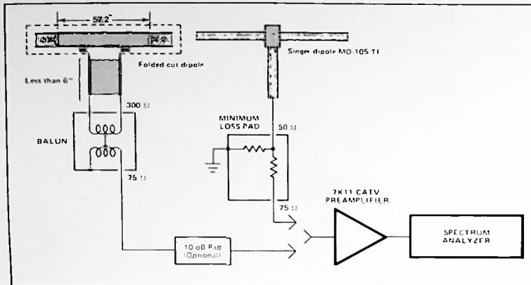
Fig. 48. Details on the construction of a Test Dipole for Fm Stations
