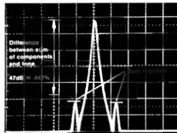
Fig. 59. Measurement Using the SMPTE Standard
