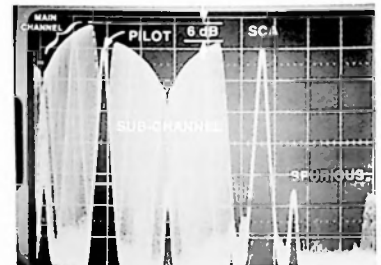
Fig. 5. Display of Composite Fm Stereo Signal on Low Frequency Spectrum Analyzer
