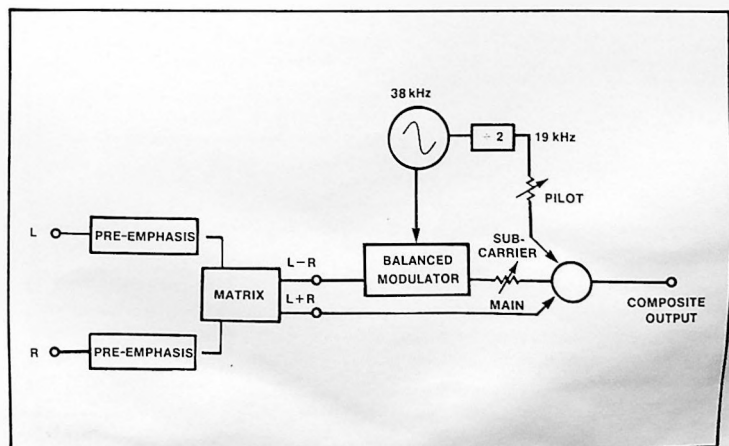
Fig. 2. Block Diagram of Theoretical Fm Stereo Generator
