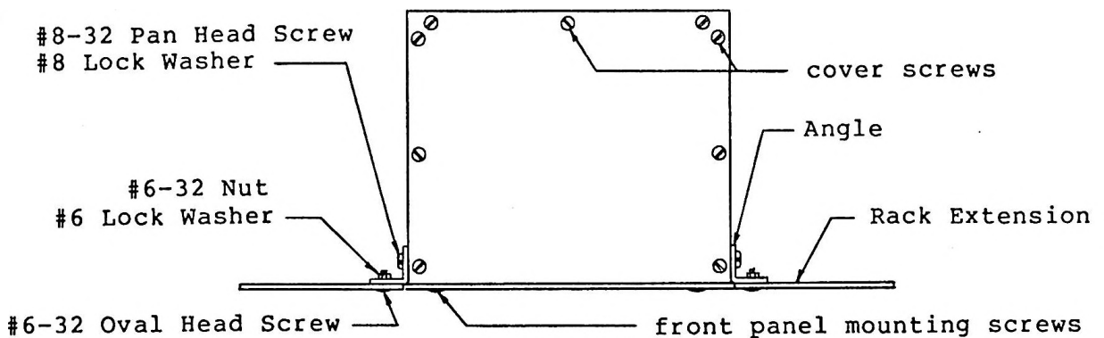
FIGURE 4. MOUNTING DETAILS FOR SR-21 RACK MOUNT KIT.
