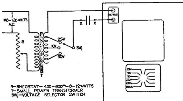
MODEL 772 ANALYZER
