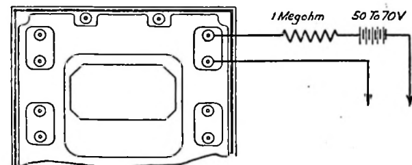
Circuit for Rx50,000 Used on Top or Rx10,000 Ohm Switch Position
