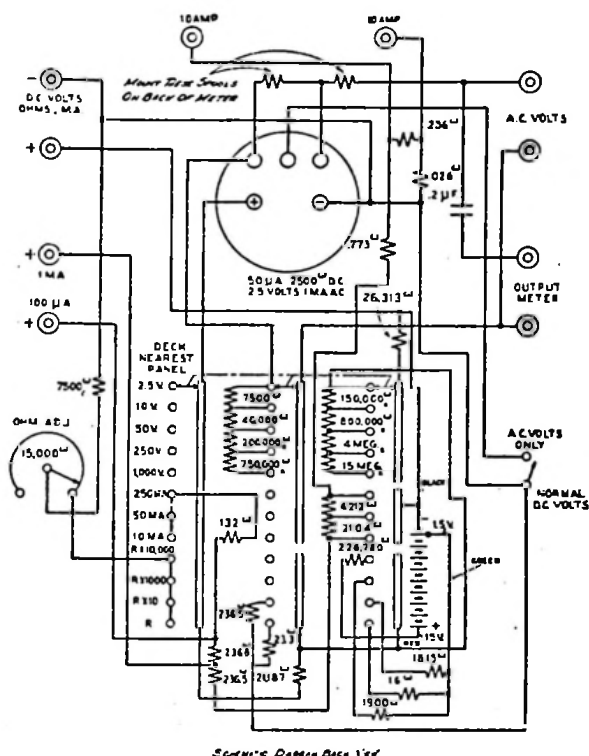
Wiring Diagram for Model 772 Analyzer
