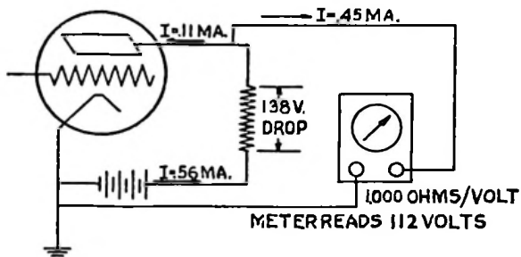
Conditions Using 1,000 Ohms Per Volt Meter
