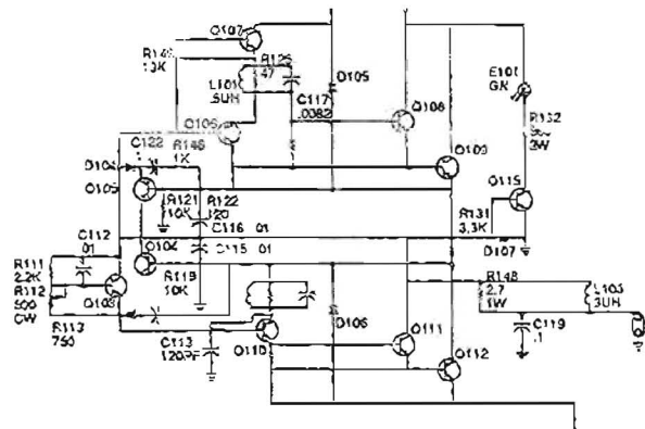
Fig. 6.5 Bias, Output and Protection Stages
